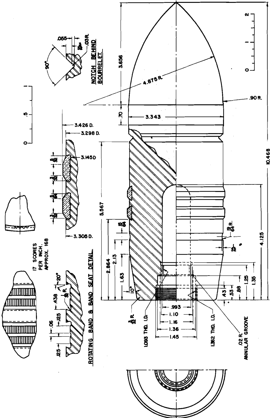
SOVIET 85MM APHE MOD. UBR-365K PROJECTILE.
