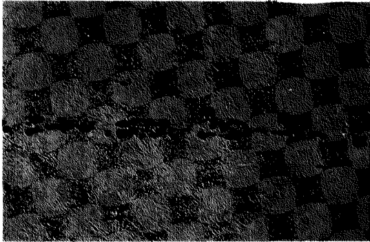
X100 -A- PICRAL FORWARD CORNER OF PROJECTILE NOSE— OXIDE TYPE INCLUSIONS AND FINE GRAINED STRUCTURE.
