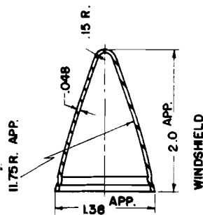
FMAM 1121 SOVIET 45MM. APHE-T MOD. UBR-243Z PROJECTILE.
