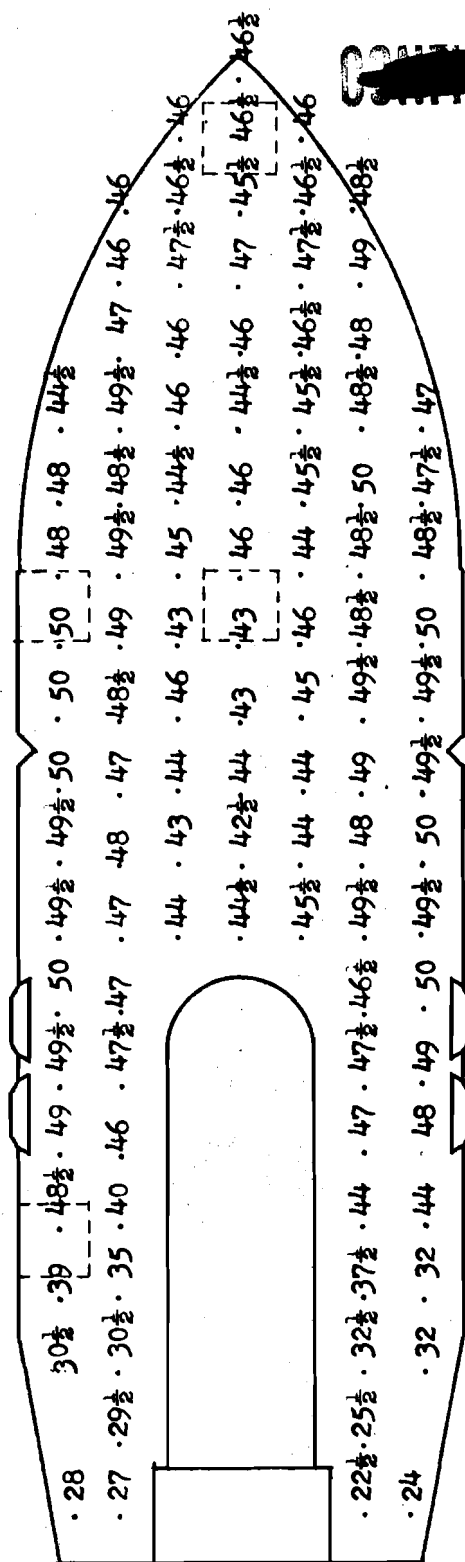
ROCKWELL C HARDNESS PATTERN ON BODY OF SOVIET 85MM APHE-T PROJECTILE MOD. UBR-365K (FMAM 2175) AND LOCATION OF SPECIMENS FOR MICROSCOPIC EXAMINATION.
