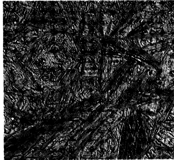
X1000 -D- PICRAL FORWARD OF EXPLOSIVE CAVITY-- SAME AREA AS C. MARTENSITE WITH TRACE OF BAINITE.
