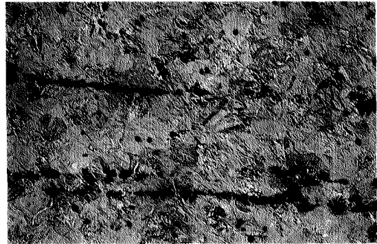
X100 -D- PICRAL CENTER OF PROJECTILE AT BOURRELET— BAD SEGREGATIONS OF OXIDE TYPE INCLUSIONS.
