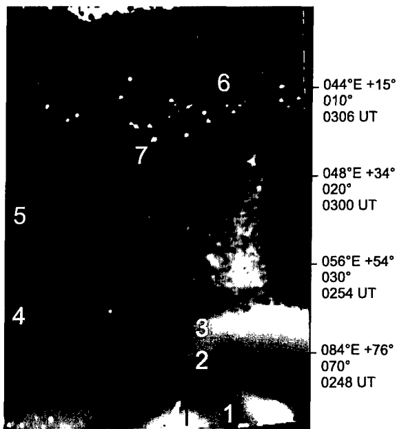
Figure 12. Streamer event observed to very low latitude, 27 July 2003. Kp equals 5 during this period and reached 6 in the previous 6 hours. The projection is similar to that in Figure 5 and covers about 80^\circ \times 110^\circ on the sidereal sky. Note that the contrast has been adjusted differentially over the image to show detail, and so the grayscale levels are not a reliable indication of relative brightness. The SMEI aurora events, as described in the text, are a bright (30 ADU) but typical streamer event at the bottom of the image, with the observation commencing about 0244 UT (1) and continuing for \sim 10 min; a very bright (90 ADU) flash event at 0248 UT (2); and the low-latitude streamer event initially observed at 0250 UT (3) and continuing for \sim 15 min down to a latitude of +20^\circ . The low-latitude streamer filaments are much fainter than the earlier events, at most a few ADU. The granular appearance from 0252 UT (4) to 0258 UT (5) is a passage through the auroral oval. The angled shadow at upper right (6) is a coronal mass ejection (CME) here observed at a solar elongation of 60^\circ . The band of speckles just prior to the CME (7) are star residuals due to a brief error in the satellite attitude determination.
