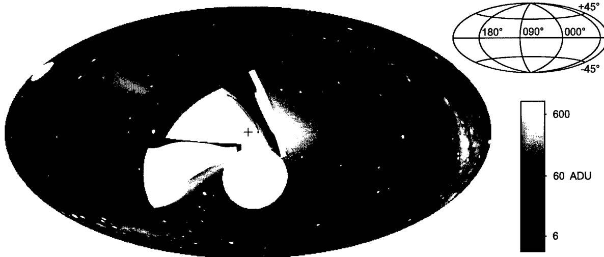
Figure 2. Example of an all-sky orbit image in a sun-centered Hammer-Aitoff projection, from 30 May 2003, 0400–0541 UT. Ecliptic coordinates are displayed at upper right. The position of the Sun is indicated with a cross. The sky-coverage gaps are the circles seen at lower center and (much distorted) at far upper left. For much of this orbit, the sunward camera is made unusable due to proximity of the Sun, either forcing the shutter to close or causing saturation. The prominent feature at upper left is an unusually bright instance of “SMEI aurora” occurring during passage through the northern polar cap. Kp equals 5 during this event but was as high as 8 in the previous 6 hours. The surface brightness of this phenomenon is about 200 ADU, greater than most of the Galactic plane.
