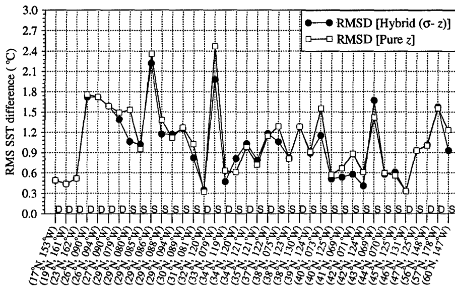
Fig. 5. SST root-mean-square difference (RMSD) between buoy and 1/8° NCOM at NODC buoys over 1 January 2000–31 March 2000. Values are calculated for \sigma - z and pure z simulations based on the daily SST time series during the 3-month period. In the x-axis, D denotes a buoy located in relatively deep water, while S denotes a buoy in comparatively shallow regions. The model is atmospherically-forced free-running and has no assimilation of any SST or other data. The reader is referred to the text for details of statistical metrics and model simulations.
