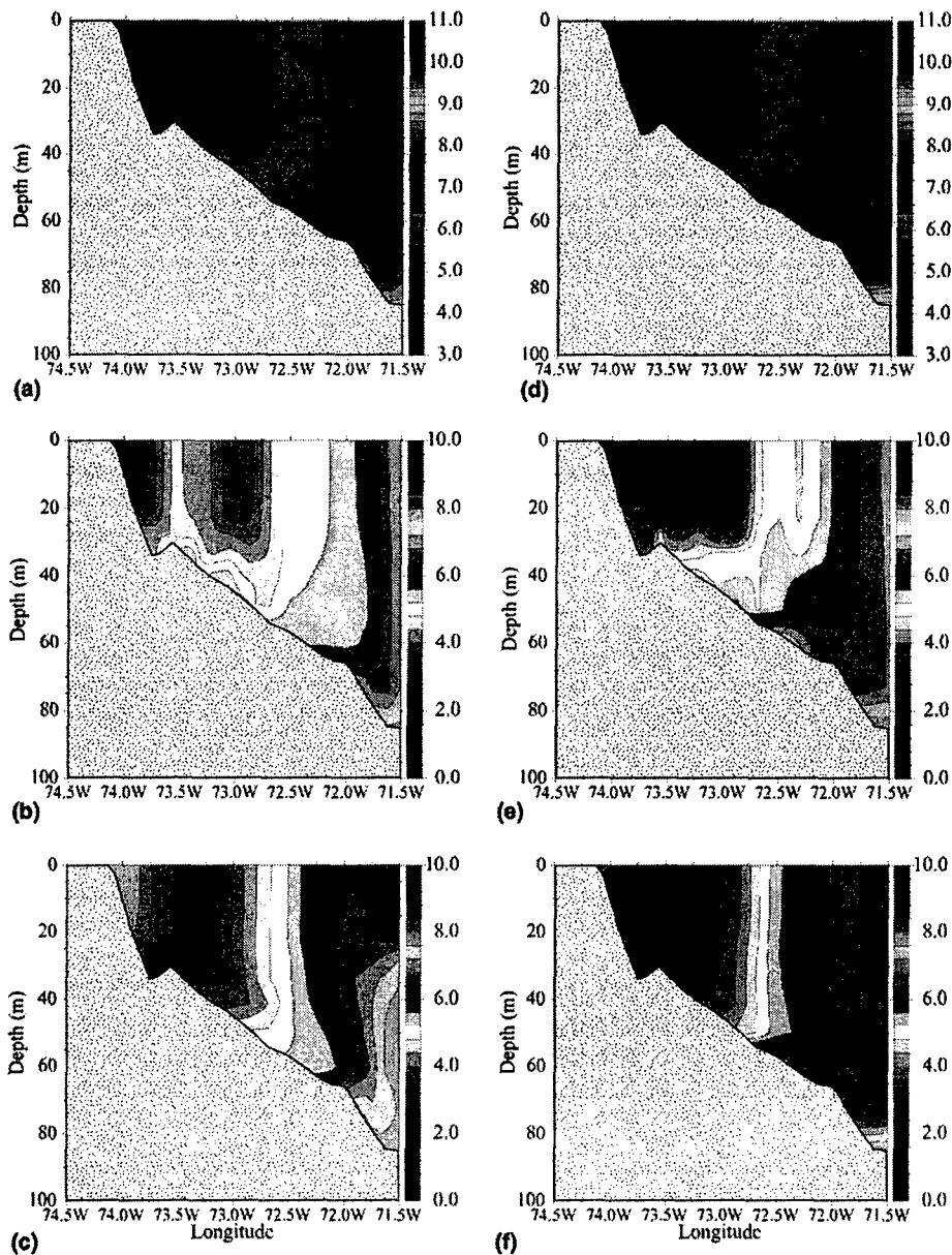
Fig. 11. Comparisons of vertical temperature sections off the eastern coast of the United States at 40.25^{\circ}\text{N} . The \sigma - z and pure z simulations show significant differences, with the \sigma - z showing better agreement with a time-series of buoy SST observation (Fig. 3). For plotting purposes, a dotted land mask is superimposed on filled temperature fields; it does not reflect the discrete steps of the z -level bathymetry that contribute to some of the differences. (a) \sigma - z simulation: January–March 2000 mean, (b) \sigma - z simulation on 11 February 2000, (c) \sigma - z simulation on 3 March 2000, (d) pure z simulation: January–March 2000 mean, (e) pure z simulation on 11 February 2000, (f) pure z simulation on 3 March 2000.
