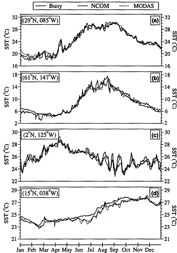
Fig. 4. Daily SST time series obtained from buoy, NCOM and MODAS at four locations in 2001: (a) an NODC buoy (29°N, 085°W), (b) a NODC buoy (61°N, 147°W), (c) a TAO buoy (2°N, 125°W) and (d) a PIRATA buoy (15°N, 038°W). Note that global NCOM assimilates 1/8° MODAS SST analysis of satellite IR data. The x -axis is labeled starting from the beginning of each month.
