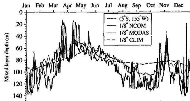
Fig. 9. Daily MLD time series obtained from buoy, NCOM and MODAS at ( 5^{\circ}\text{S} , 155^{\circ}\text{W} ). ME values between buoy vs. NCOM, MODAS and MODAS climatology are -9 , -14 and -13 m, and R values are 0.74 , 0.77 and 0.69 , respectively.
