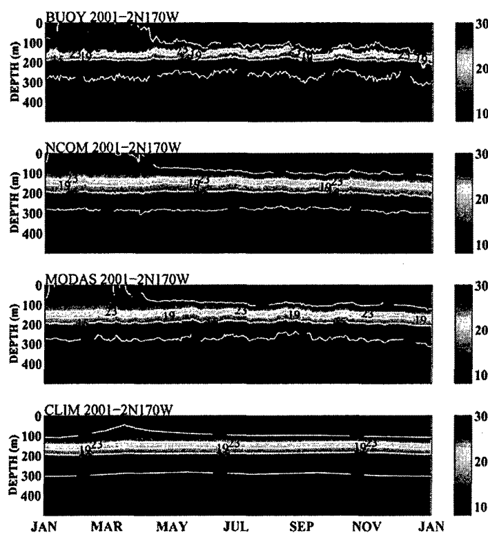
Fig. 5. Spatial daily subsurface temperature variability ( ^{\circ}\text{C} ) obtained from buoy, NCOM and MODAS and MODAS climatology at a TAO buoy, ( 2^{\circ}\text{N} , 170^{\circ}\text{W} ), located in the equatorial Pacific Ocean. All are in 2001, and the water depths at which buoy subsurface measurements were taken are at 1, 25, 50, 75, 100, 125, 150, 200, 250, 300, and 500 m. Accuracy of subsurface temperatures reported from the buoy is 0.03^{\circ}\text{C} . Note that global NCOM assimilates 1/8^{\circ} MODAS subsurface temperatures. The x-axis is labeled starting from the beginning of each month.
