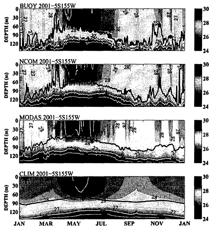
Fig. 8. Spatial daily MLD variability (thick black line) superimposed on daily subsurface temperatures ( ^{\circ}\text{C} ) obtained from buoy, NCOM and MODAS and MODAS climatology at a TAO buoy, ( 5^{\circ}\text{S} , 155^{\circ}\text{W} ), located in the central Pacific Ocean in 2001. Kara et al. (2000a) provides details of MLD calculations presented in this paper.
