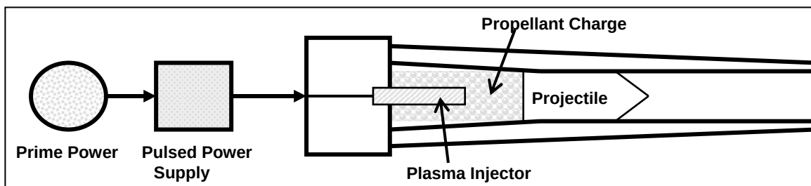
Figure 13. Simplified schematic of ETC propulsion gun.
