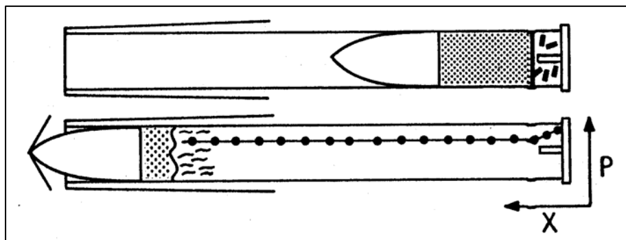
Figure 19. Schematic of traveling charge propulsion concept (40).
