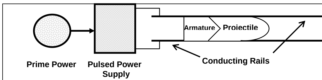
Figure 23. Simplified schematic of electromagnetic gun – railgun concept.
