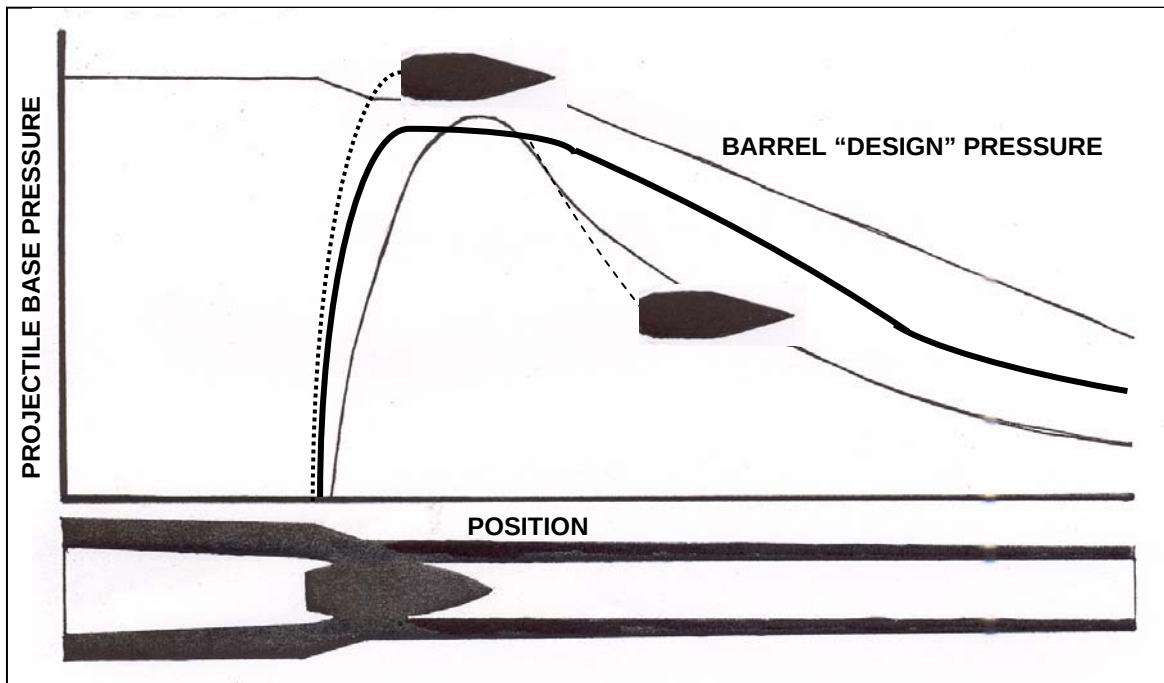
Figure 2. The challenge for more performance: increasing the area under the pressure vs. travel curve without exceeding system pressure limits.
