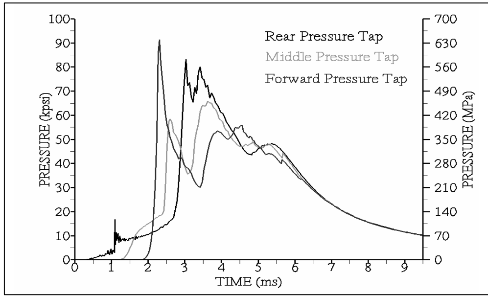
Figure 5. Predicted pressure vs. time profiles for nominal telescoped ammunition (12).
