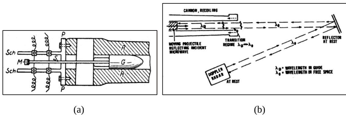
Figure 4. (a) Projecting rod technique (4); (b) microwave interferometry (5).
