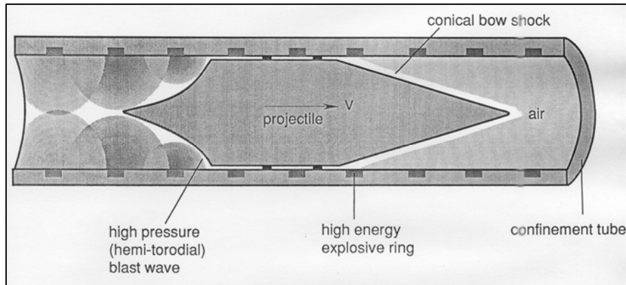
Figure 18. Detonation wave acceleration from explosive lined tube (38).
