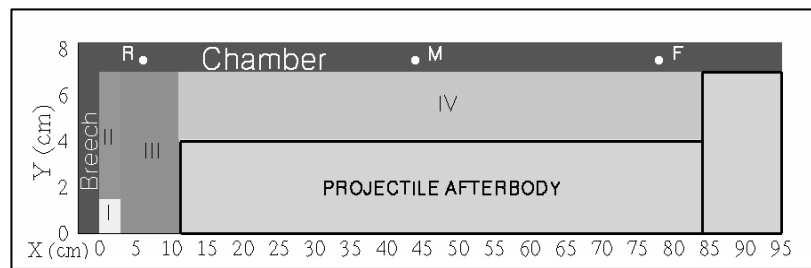
Figure 8. Schematic (axisymmetric half figure) of nominal telescoped ammunition (12).
