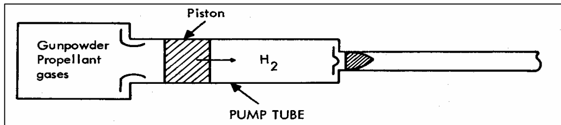
Figure 21. Simplified schematic of single-stage light gas gun (44).
