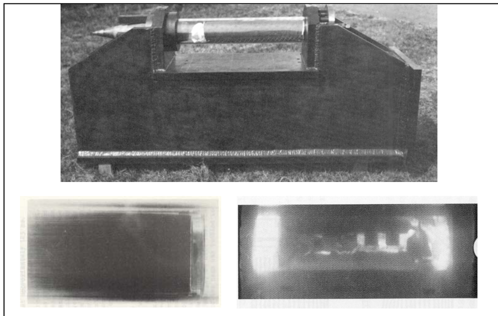
Figure 6. The 155-mm chamber simulator, flash radiograph, and cinematographic frame (11).
