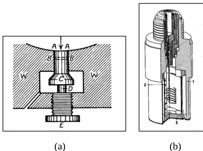
Figure 3. (a) Noble crusher gage (4); (b) piezoelectric crystal gage (2).
