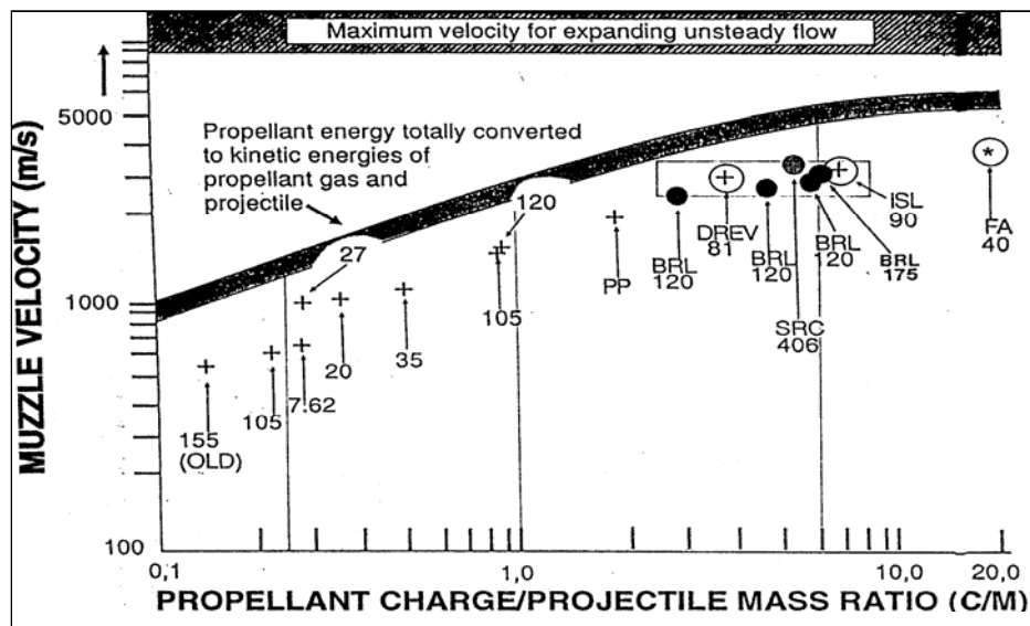
Figure 14. Experimental and predicted muzzle velocities as a function of propellant charge to projectile mass ( C/M ) (based on reference [30] and updated by Horst).
