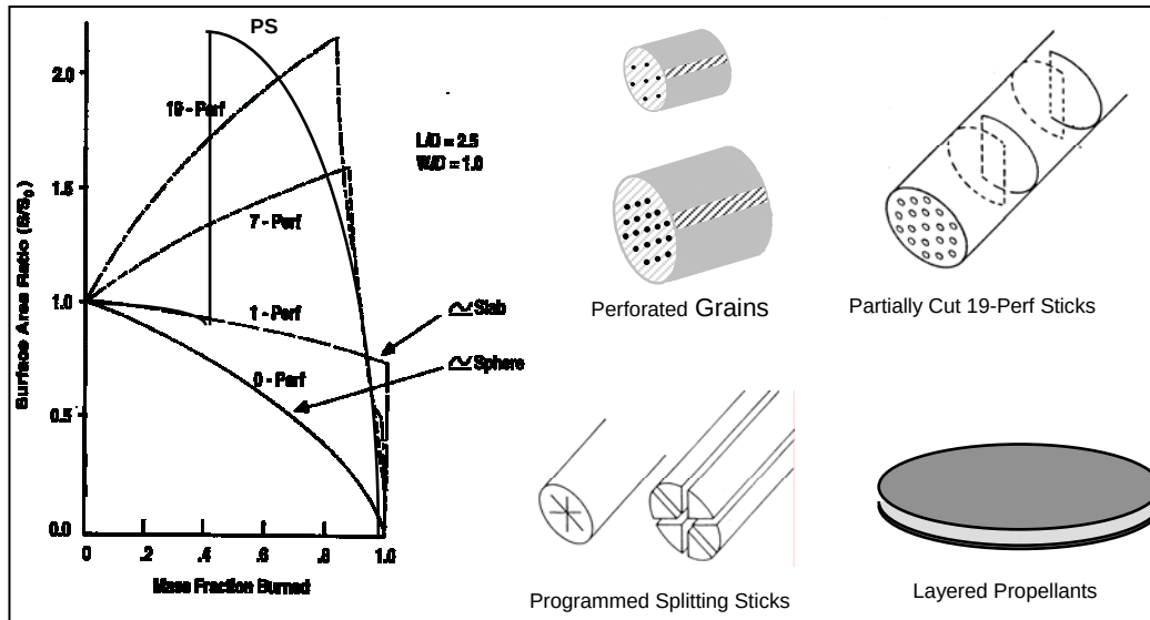
Figure 10. Progressivity and geometry of various propellant configurations (1).
