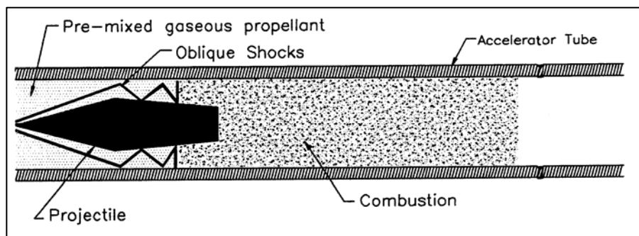
Figure 20. Schematic of inbore ram accelerator concept (thermally choked mode) (43).
