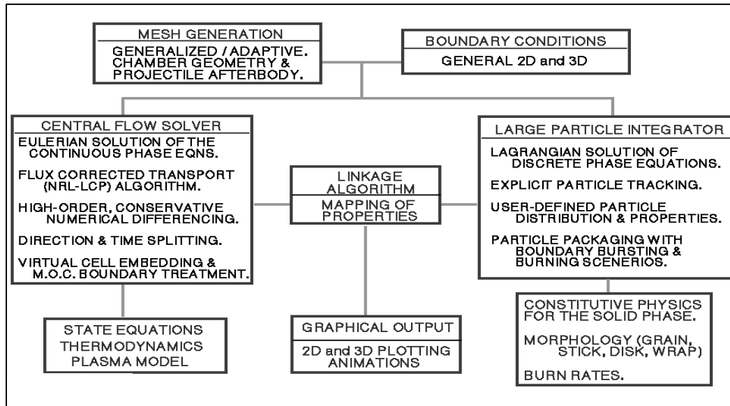
Figure 7. Schematic of NGEN3 multidimensional multiphase flow interior ballistics code (21).
