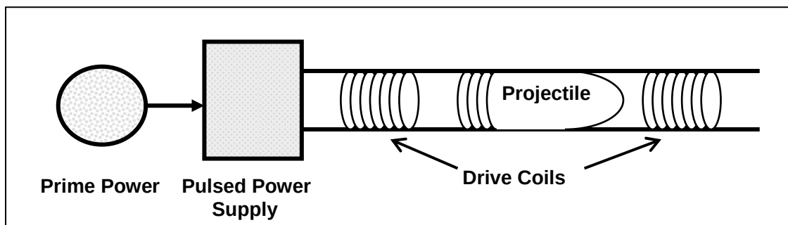
Figure 22. Simplified schematic of electromagnetic gun – coilgun concept.
