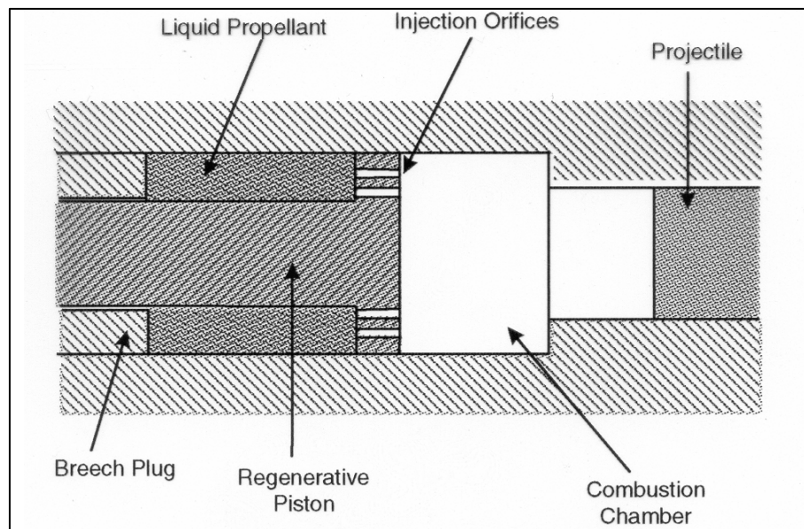
Figure 12. Simplified schematic of regeneratively injected liquid propellant gun.
