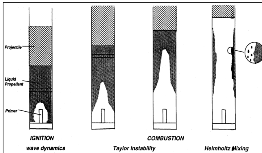
Figure 11. Conceptual interior ballistic process for bulk-loaded liquid propellant gun.
