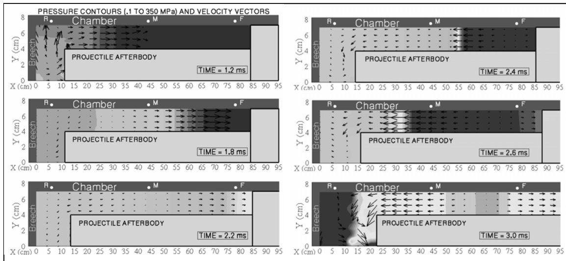
Figure 9. Predicted gas velocity and pressure fields for nominal telescoped ammunition (12).
