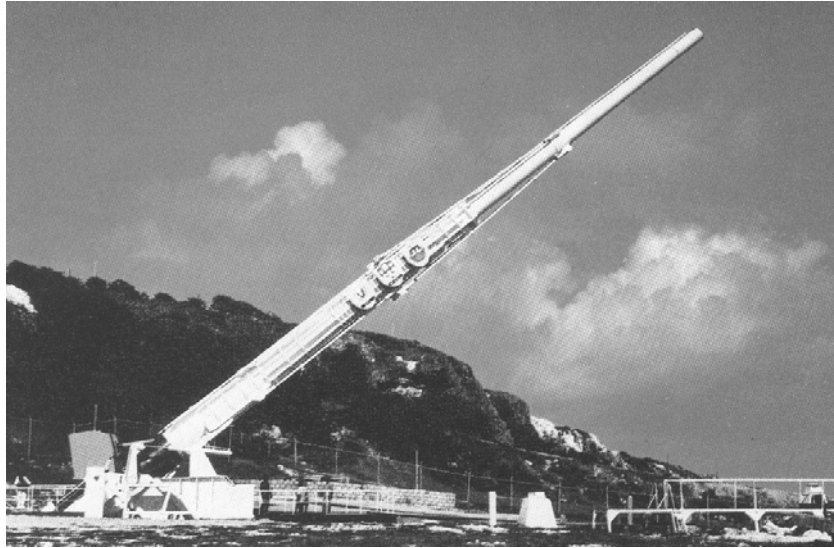
Figure 16. The 16-in, 86-cal HARP Gun – 1965 (32).
