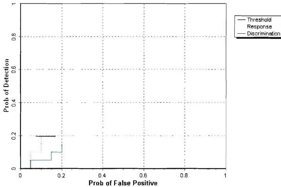
Figure 2. GEM-3 wooded area probability of detection for response and discrimination stages versus their respective probability of false positive over all ordnance categories combined.
