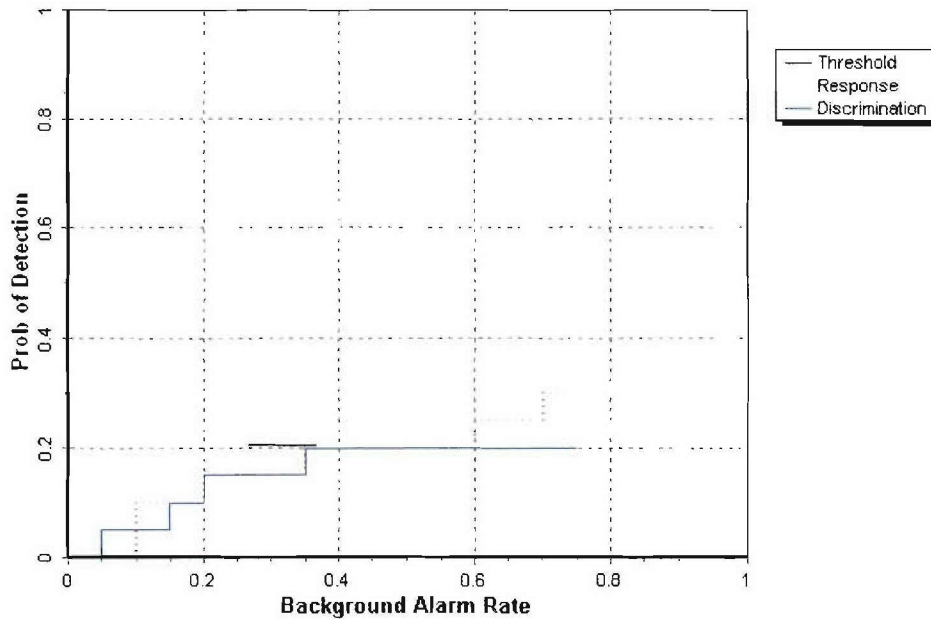
Figure 5. GEM-3 wooded area probability of detection for response and discrimination stages versus their respective background alarm rate for all ordnance larger than 20 mm.
