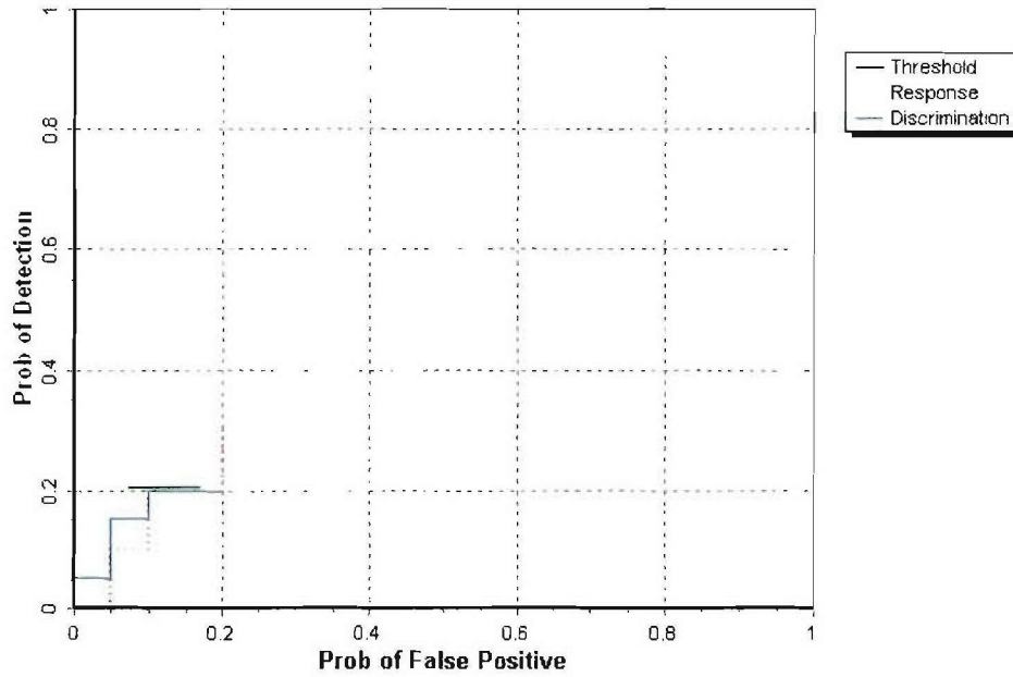
Figure 4. GEM-3 wooded area probability of detection for response and discrimination stages versus their respective probability of false positive for all ordnance larger than 20 mm.
