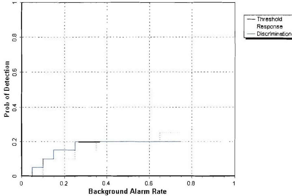
Figure 3. GEM-3 wooded area probability of detection for response and discrimination stages versus their respective background alarm rate over all ordnance categories combined.
