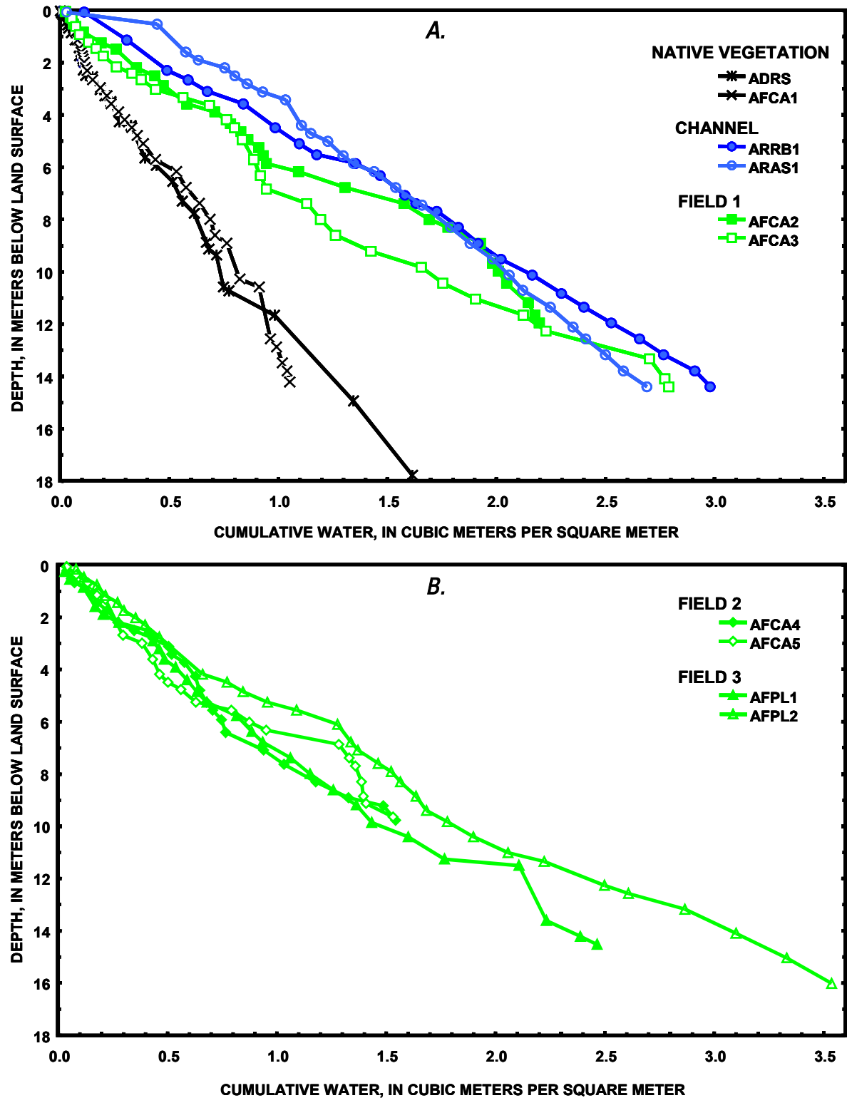
Figure 7. Profiles of cumulative water beneath irrigated fields, the Amargosa-River channel, and native vegetation, Amargosa Desert, Nye County, Nevada. A. Native-vegetation, channel, and newest-field (irrigated since 1993) boreholes. B. Older-field (irrigated since the 1960's) boreholes. See fig. 2 for locations.
