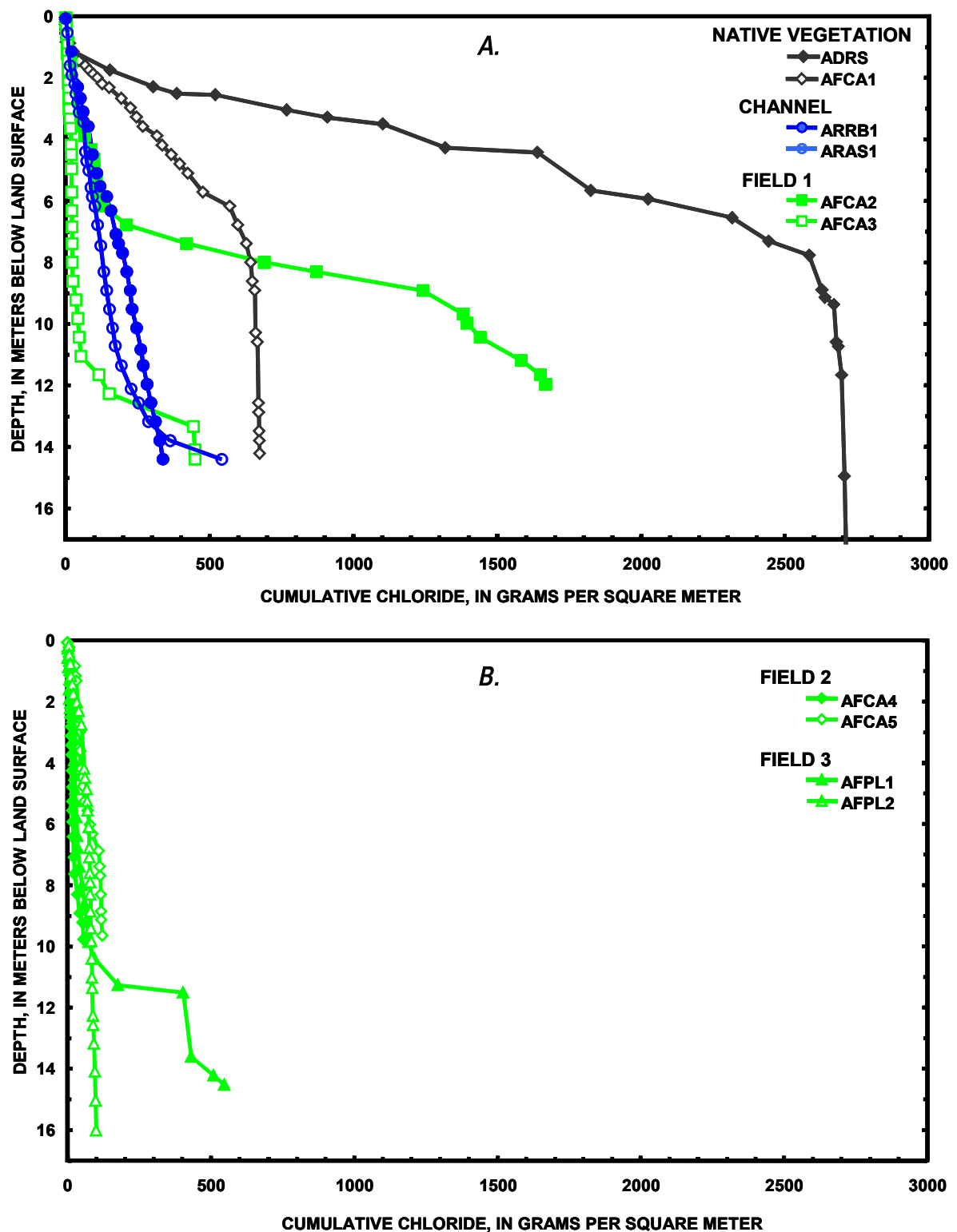
Figure 8. Profiles of cumulative chloride beneath irrigated fields, the Amargosa-River channel, and native vegetation, Amargosa Desert, Nye County, Nevada. A. Native-vegetation, channel, and newest-field (irrigated since 1993) boreholes. B. Older-field (irrigated since the 1960's) boreholes. See fig. 2 for locations.
