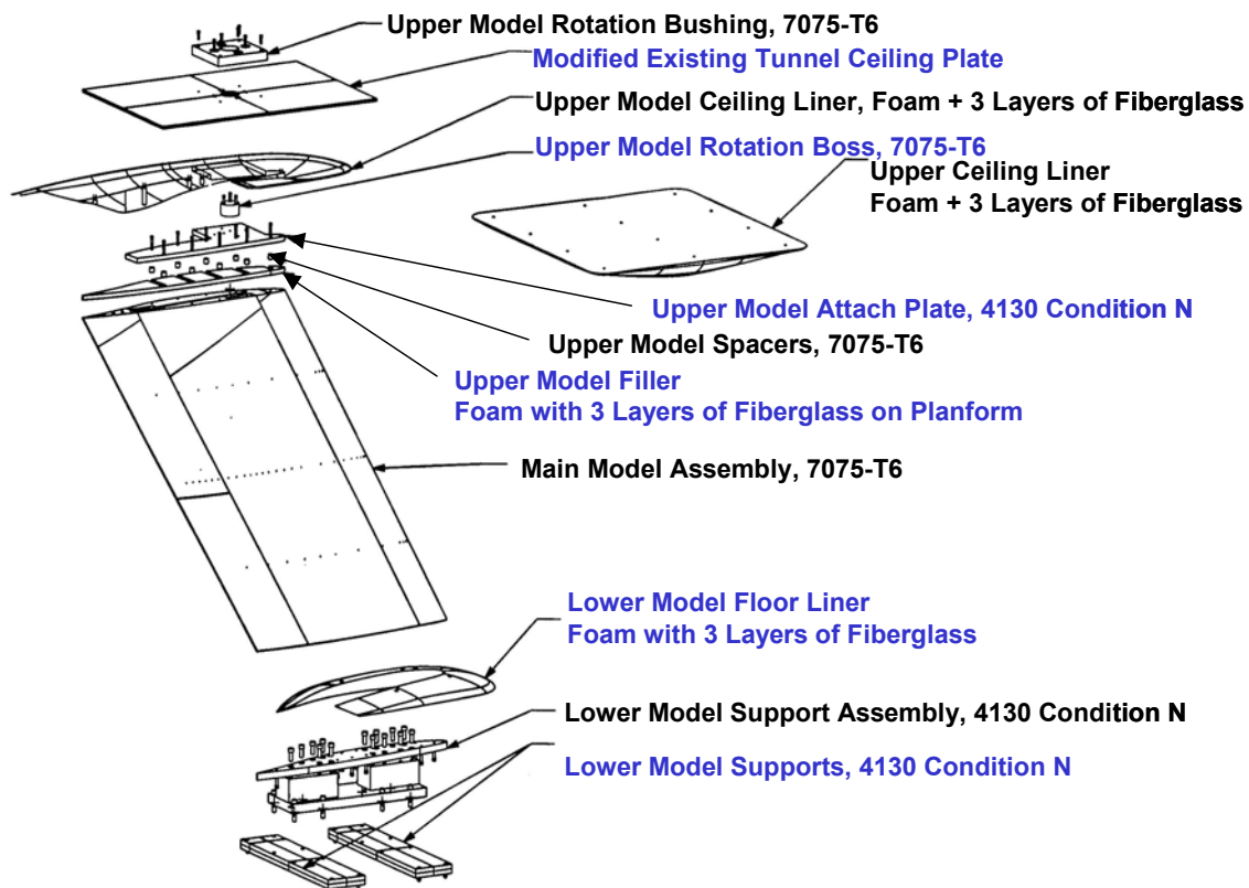
Figure 26: Exploded View of Model Assembly
