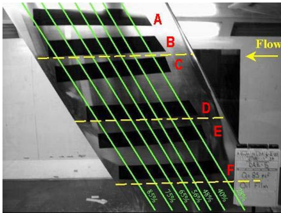
Figure 32: Mylar Strips and Reference System for Oil Film Interferometry
