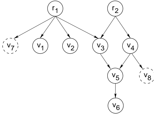
Figure 8: View Dependency Graph for the Motivating Example
