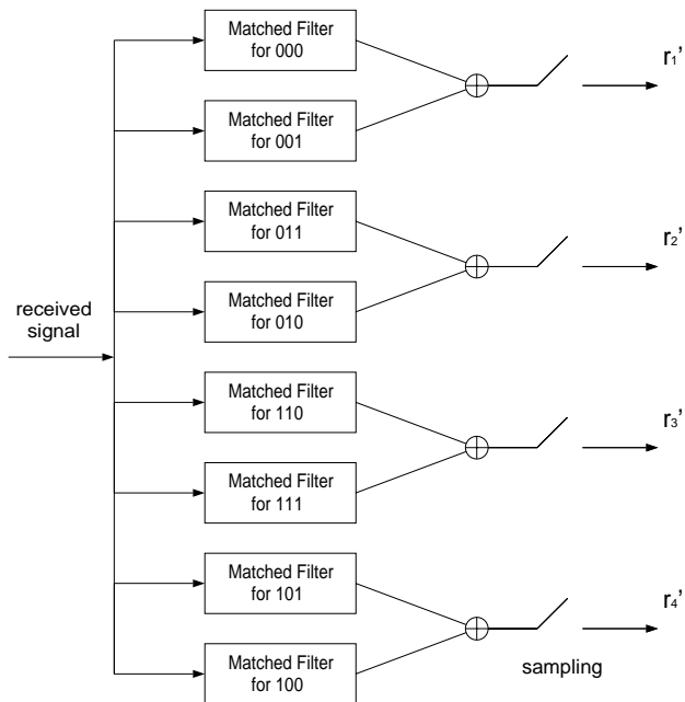
Figure 2: Modified optimum receiver for passive rate control. The received signal is projected to the sum of the adjacent signals.
