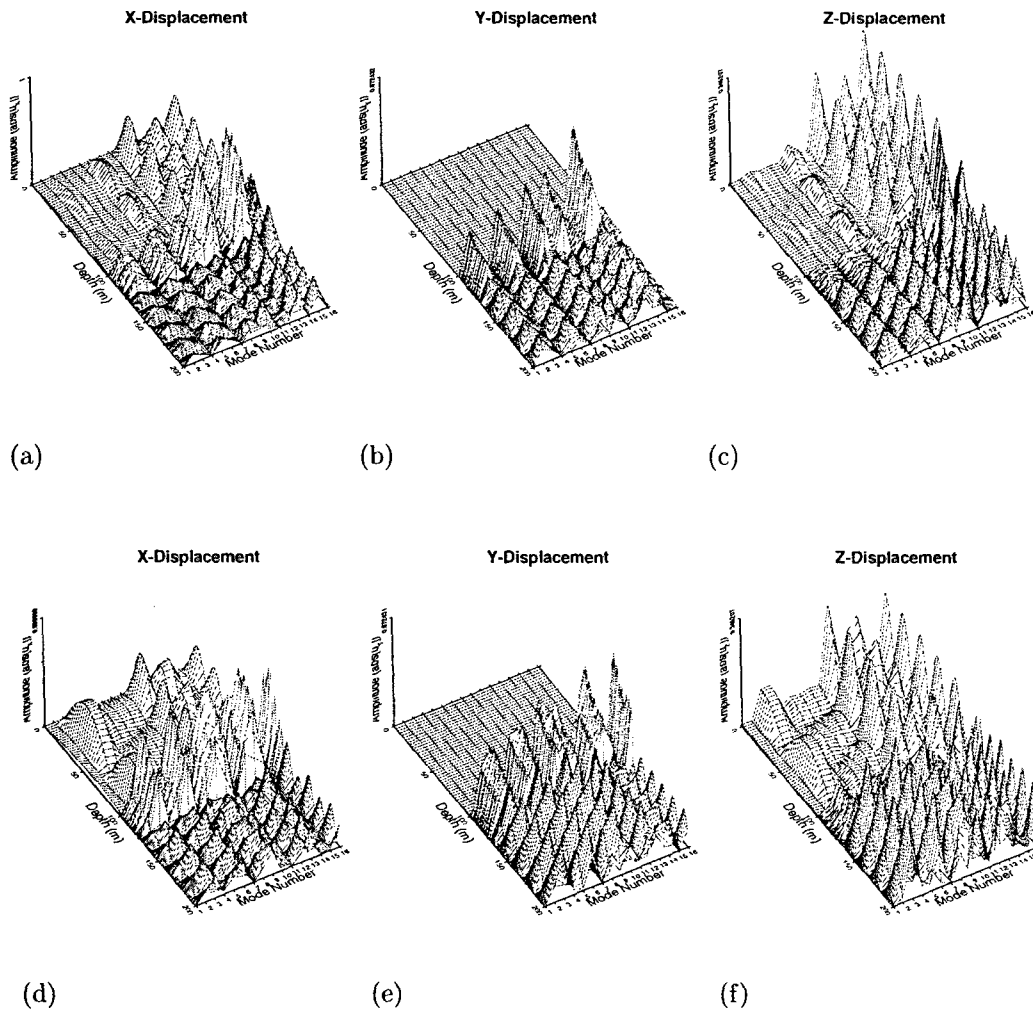
Figure 19: Both explosive and double couple sources are effective at exciting modes with 3-D particle motion. This is purely a result of the introduction of anisotropy into the sediments, which results in the coupling of the x, y, and z particle displacements. Note that the double couple source is more effective at exciting the lower order modes, than the explosive source. The figures show the displacement of all the modal eigenfunctions with phase velocities between the of 1500m/s and 2000m/s. The x, y and z-components of displacement are shown in figures (a) & (d), (b) & (e), and (c) & (f) respectively. P-SV-SH modes are clearly evident with energy in all three coordinate directions.
