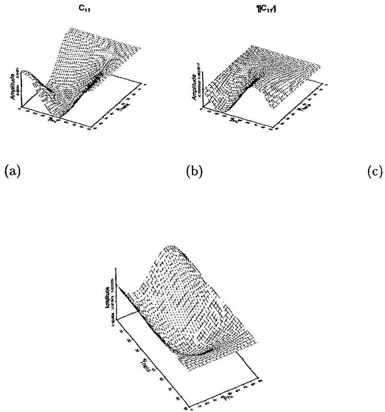
Figure 3: The C_{11} element of the elastic stiffness matrix {}^a C_{IJ} is shown in Figure 3(a) for various angles of \theta and \varphi . This is a numerical plot of equation 11. Figures 3(b) and 3(c) plot the sensitivity of the C_{11} element to the angles \varphi and \theta respectively.
