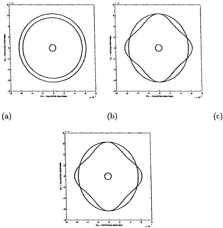
Figure 7: The slowness curves for the xy , xz , and yz -planes for a VTI anisotropic sediment layer, where \hat{s} = \hat{z} . The inner circle is the compressional slowness, indicating the absence of any anisotropy in the compressional velocity. The outer paths represent the vertical and horizontal shear slownesses. In Figure (a) there is complete shear velocity splitting. Both Figures (b) and (c) reveal shear velocity singularities at \theta = 0^\circ, 180^\circ and \theta \approx 70^\circ, 110^\circ .
