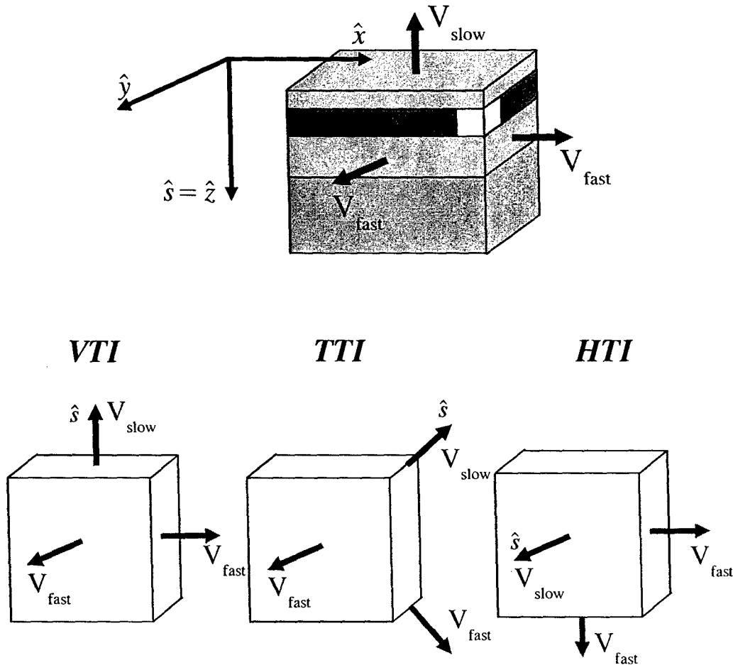
Figure 1: A representative elastically symmetric transversely isotropic structure (TI) due to compositional layering with a vertical symmetry axis \hat{s} . The fast velocity directions V_{fast} are normal to the symmetry axis direction and parallel to the bedding plane, the xy -plane for this instance. The slow velocity direction V_{slow} is parallel to the vertical symmetry axis. A TI structure with a vertical symmetry axis is often referred to as vertical transverse isotropy (VTI) or as azimuthally isotropic. The geometrical orientation of the anisotropy in a plane layered homogeneous anisotropic model, depends on the orientation of the symmetry axis \hat{s} . The white block of material from the plane layered structure on the right is expanded on the left to show the importance of symmetry axis direction on velocity properties of the medium. A structure can be transversely isotropic with a vertical, tilted (neither vertical nor horizontal), or horizontal symmetry axis and be classified as VTI, TTI, or HTI respectively. For a VTI orientation, the fast velocity direction is in the horizontal plane. A TTI orientation results in the fast velocity direction being contained to an oblique plane and the HTI orientation restricts the fast velocity directions to a vertical plane normal to the symmetry axis \hat{s} . Note that the slow velocity direction ( V_{slow} ) always corresponds with the symmetry axis direction \hat{s} .
