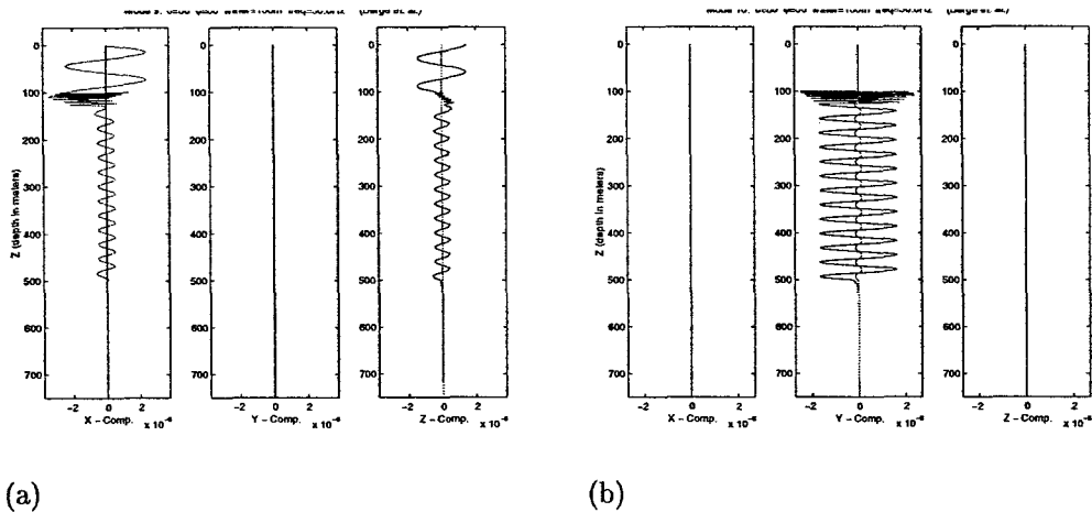
Figure 12: This is an example of P-SV and SH modes for \hat{s}(\theta, \varphi) = \hat{s}(80^\circ, 0^\circ) . This is an instance where the elastic stiffness matrix is quasi-monoclinic and the pure P-SV and SH modes have completely separate polarizations. The P-SV mode has particle motion in the sagittal plane and the SH mode has particle motion in the y-coordinate-direction of the horizontal plane.
