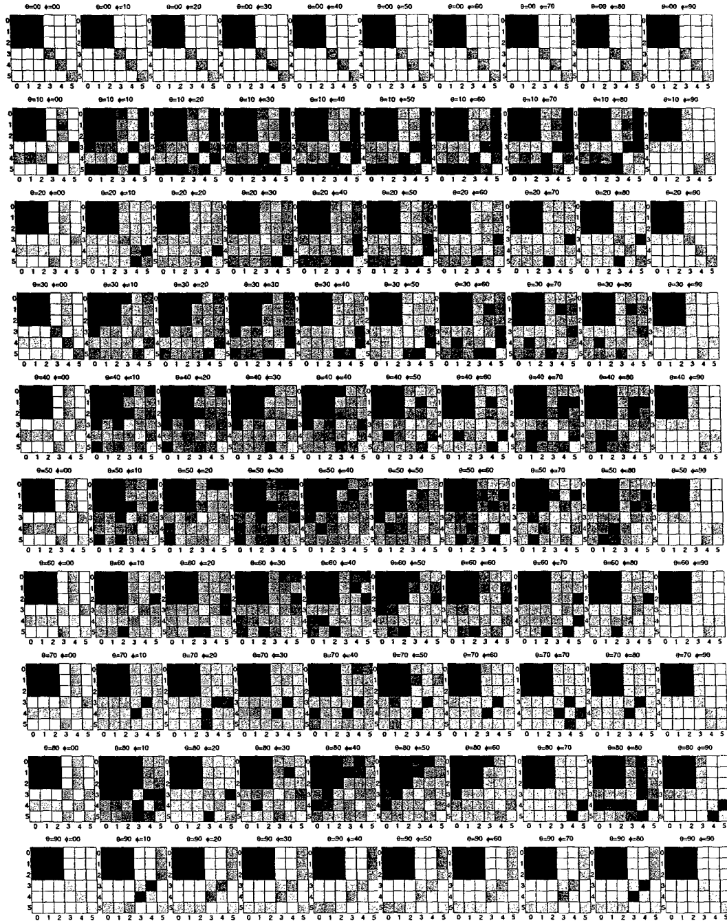
Figure 27: Each matrix in the figure represents the form of the elastic stiffness matrix {}^aC_{IJ} for specific orientations of the symmetry axis \hat{s} . The matrices graphically reveal how the elastic stiffness matrix {}^aC_{IJ} is populated as the symmetry axis is rotated. Each matrix in a horizontal row represents a 10^\circ increments in \varphi for a fixed value of \theta . Likewise, each matrix in a vertical column represents a 10^\circ increment of \theta for a fixed value of \varphi . The first row represents rotations about the y-axis, the last row represents rotations about the x-axis, and the last column represents rotations about the z-axis when \hat{s} is within the xy-plane. All of the matrices on the outside edges of the figure represent the elastic stiffness matrix being rotated about a coordinate axis and have a quasi-monoclinic form. More general rotations of the symmetry axis \hat{s} results in a quasi-triclinic form of {}^aC_{IJ} .
