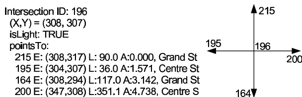
Figure 5: Intersection Representation
