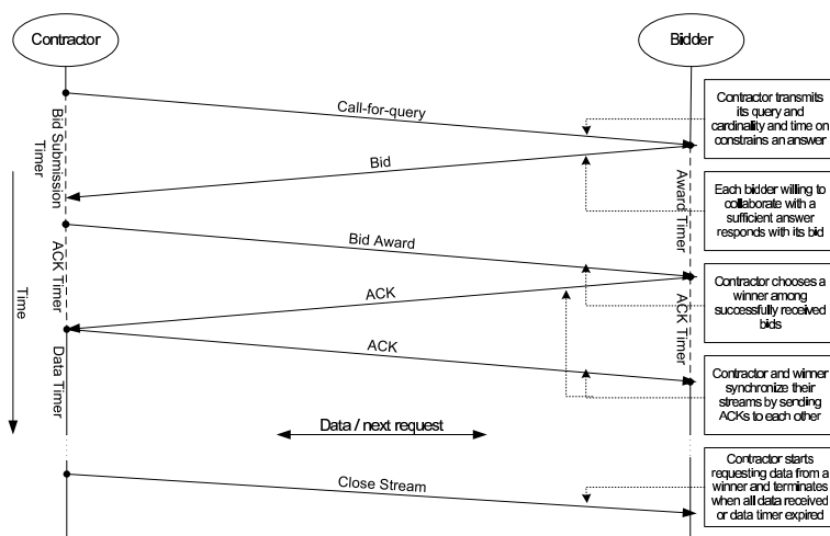
Figure 3: Message and state flow in the Collaborative Query Processing protocol
