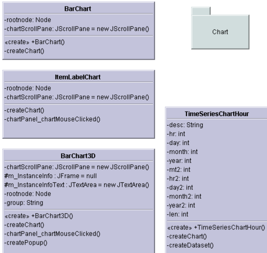
Figure 51: Classes in edu.memphis.issrl.secon.gui.chart package
