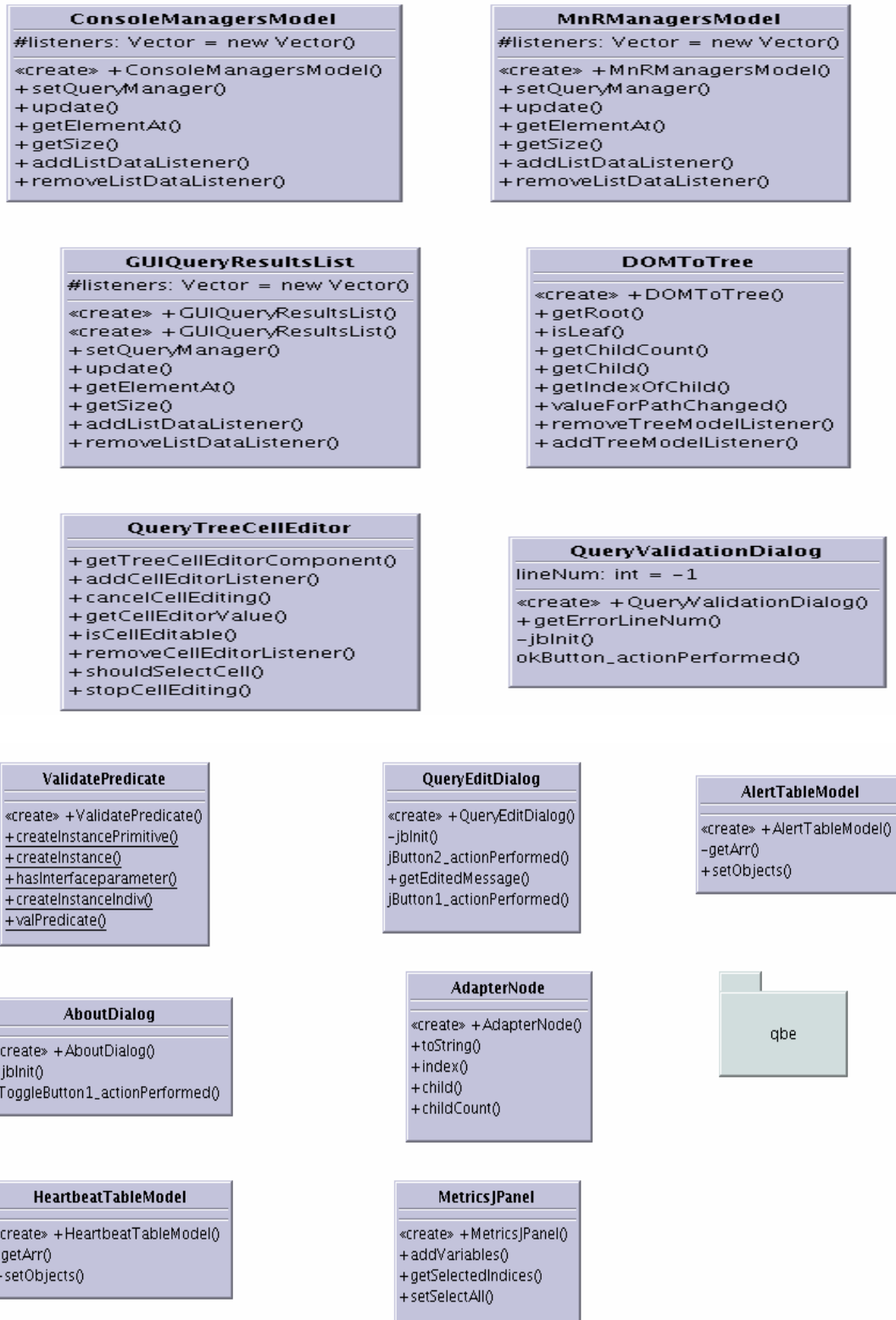
Figure 50: Classes in edu.memphis.issrl.secon.gui package
