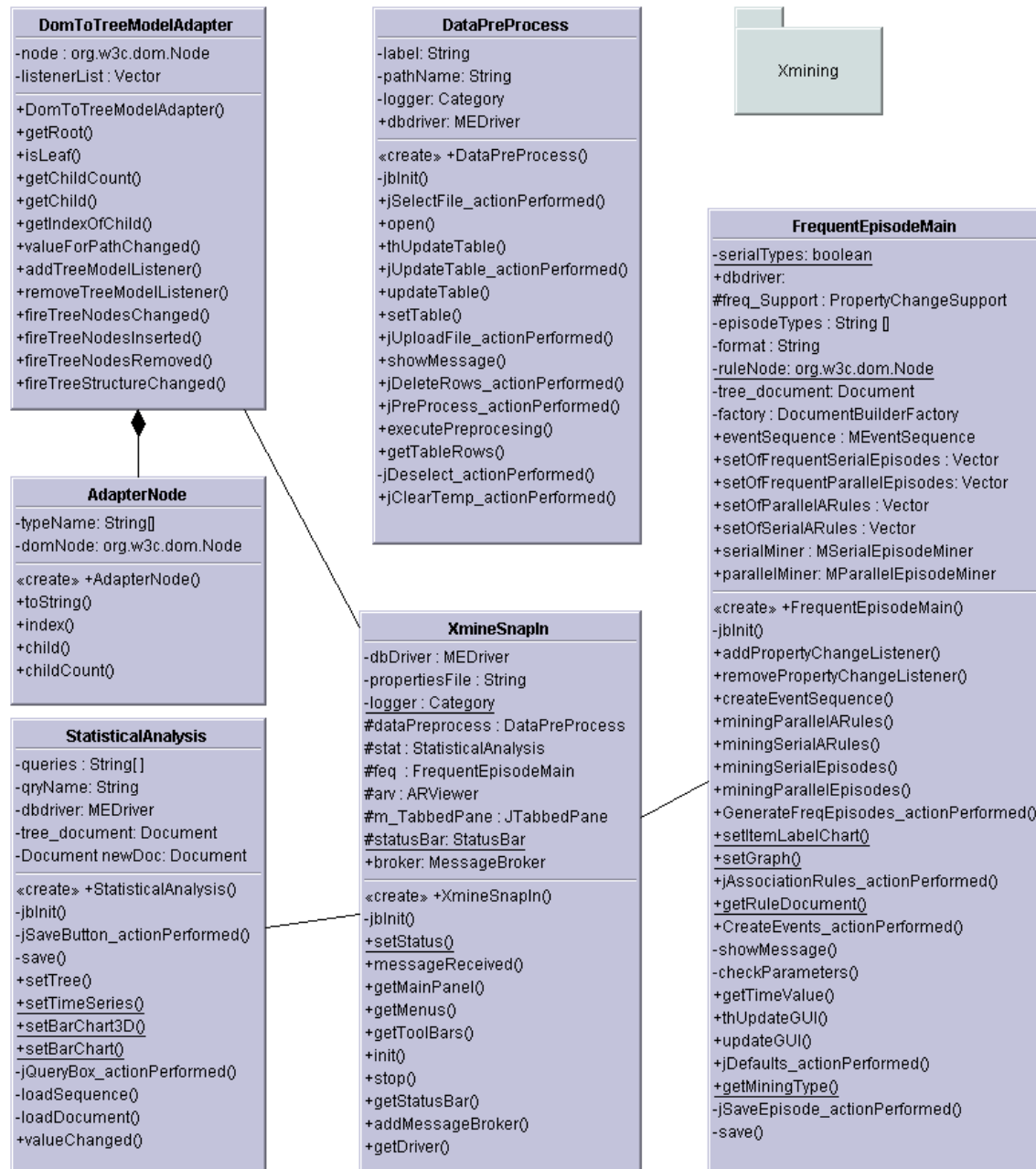
Figure 53: Classes in edu.memphis.issrl.secon.gui.Xmining package
