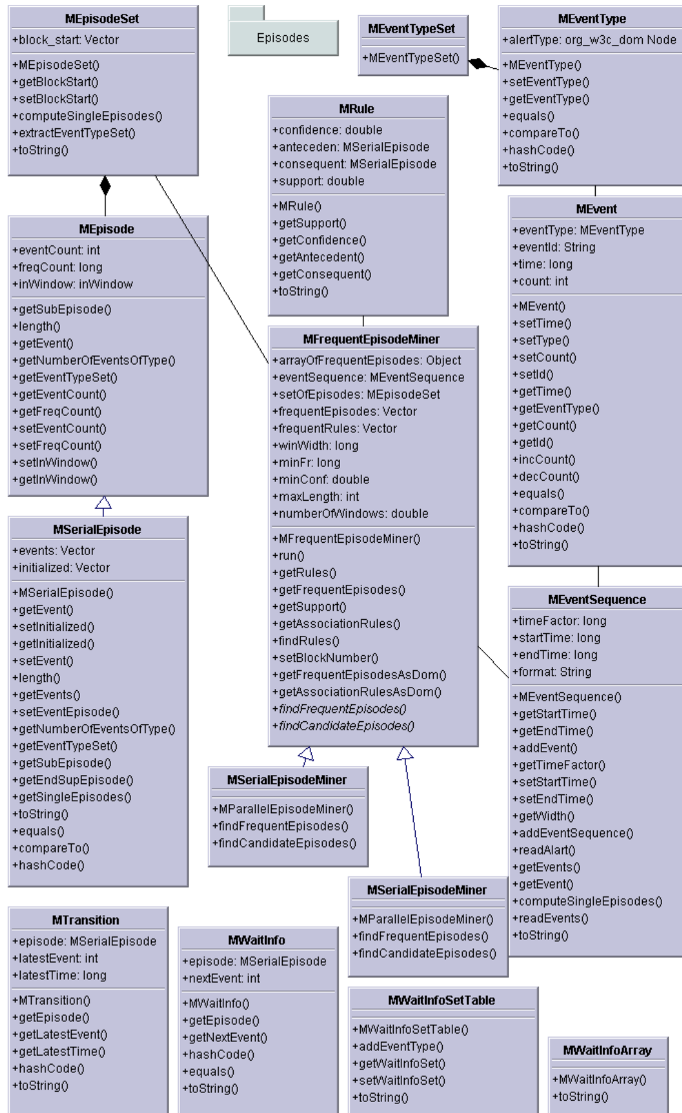
Figure 64: Classes edu.memphis.issr.secon.Xmining.Episodes package
