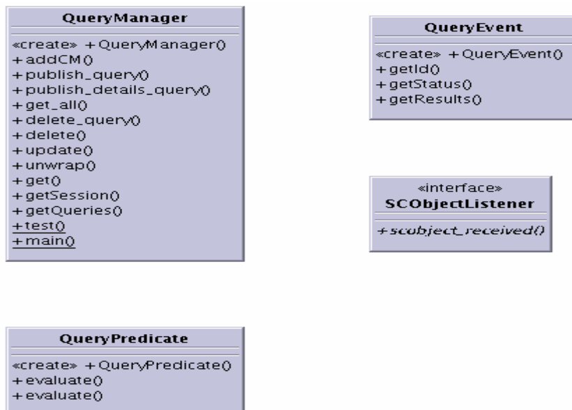
Figure 60: Classes in edu.memphis.issrl.secon.querymanager classes
