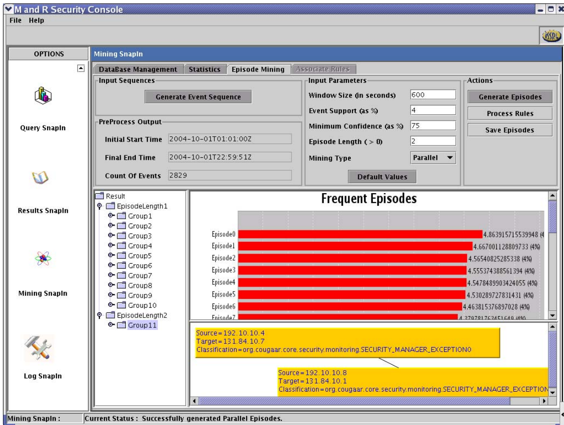
Figure 43: Episode Mining showing the Frequent Episodes for the Parallel Mining. The tree View shows the groups for each Length Type. The upper chart shows the count of each Episode and its percentage distribution. The lower chart depicts the two events for the length two Episode and the event details.
