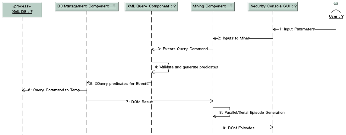
Figure 12: Initialize Mining Sequence
