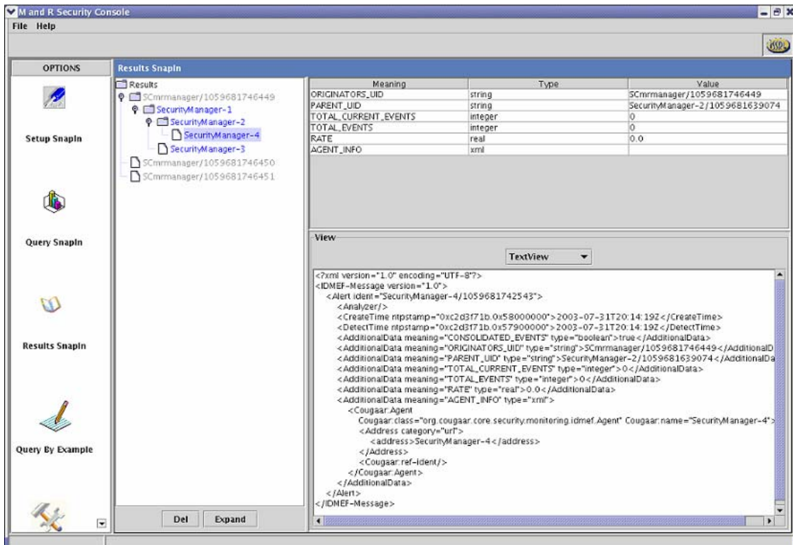
Figure 28: Results for a Security Agent in Text View
