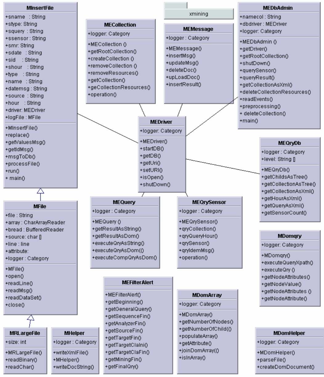
Figure 63: Classes edu.memphis.isrsl.secon.Xmining package
