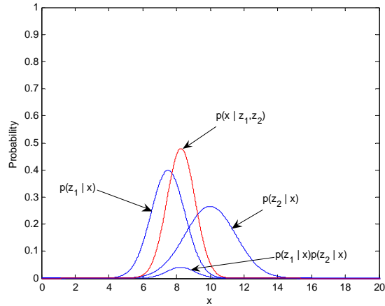
Fig. 4. Fusion of Two Gaussian Distributions
