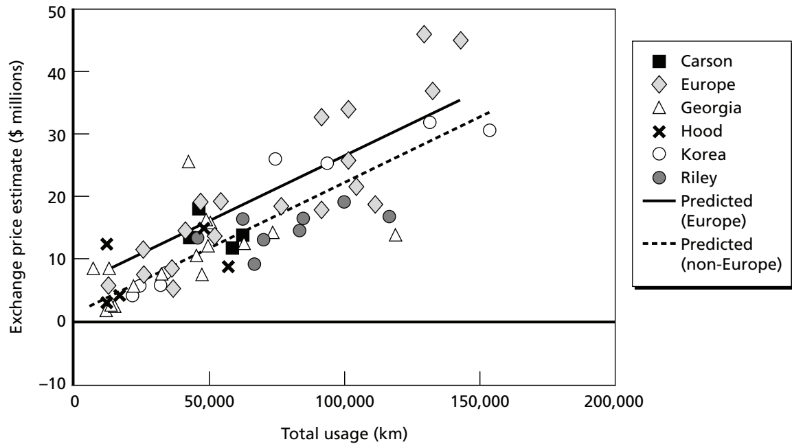
Figure D.4 Total Usage Is a Significant Predictor of the M1A1 Exchange Price Valuation of Spare Part Costs
