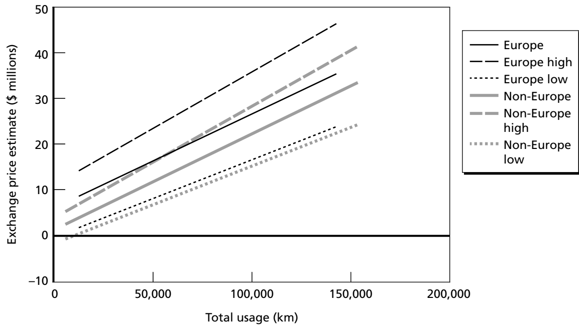
Figure D.5 Predicted M1A1 Exchange Price Estimate Versus Total Usage, by Location
