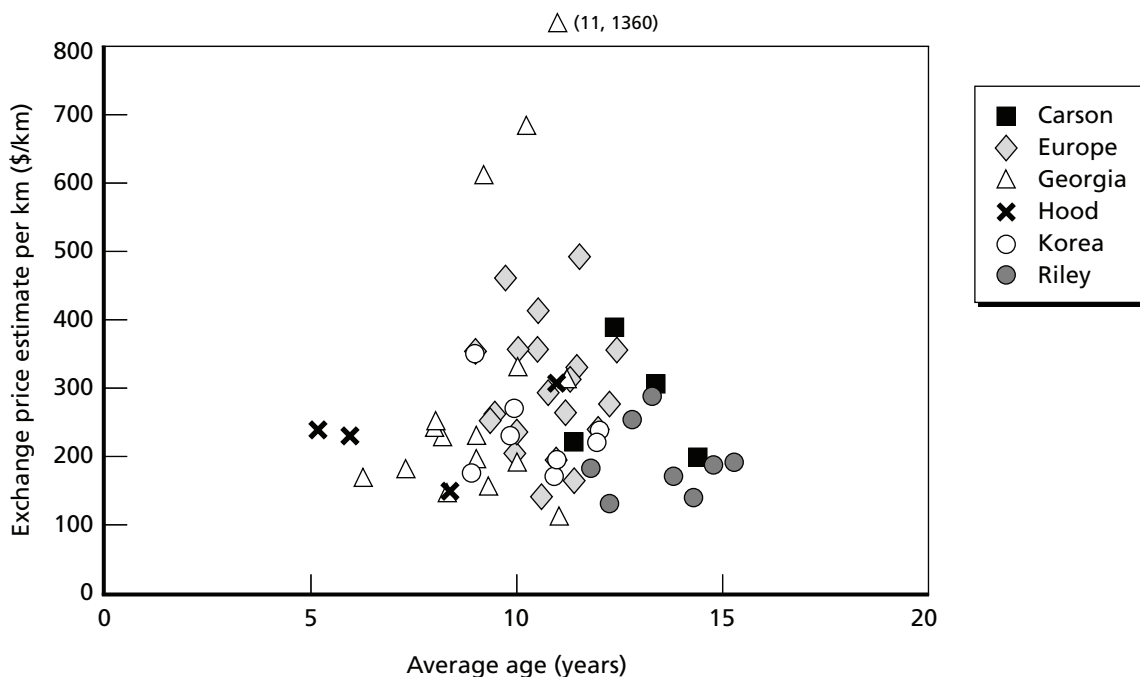
Figure S.2 Average Age Does Not Positively Affect M1A1 Exchange Price Estimate When Adjusted for Total Usage
