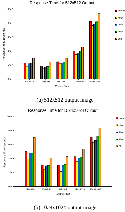
Fig. 5. Performance results for the Virtual Microscope ADR server running on 5 processors for varying image chunk sizes. Average response times of the server for the queries to produce an output image.
