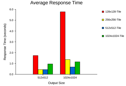
Fig. 16. Overall average response times of caching client for varying cache tile sizes.
