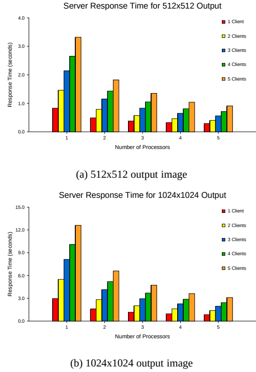
Fig. 6. Performance figures for Virtual Microscope ADR server on varying number of processors for generating the output image. In this experiment, each client submits 100 queries to the server.
