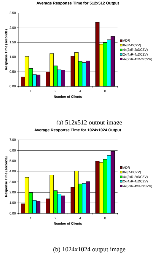
Fig. 13. Average response time of different versions of the VM servers on the 8-processor SMP.
