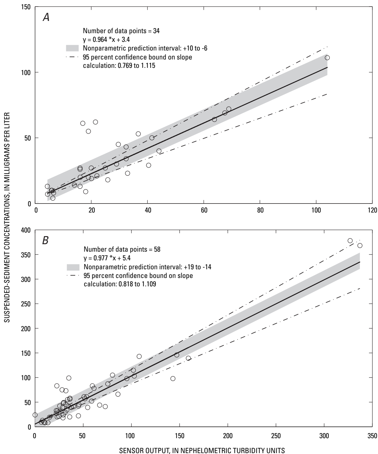
Figure 9. Calibration of (A) mid-depth and (B) near-bottom optical backscatterance sensors at Carquinez Bridge, San Pablo Bay, California, water year 2002.
