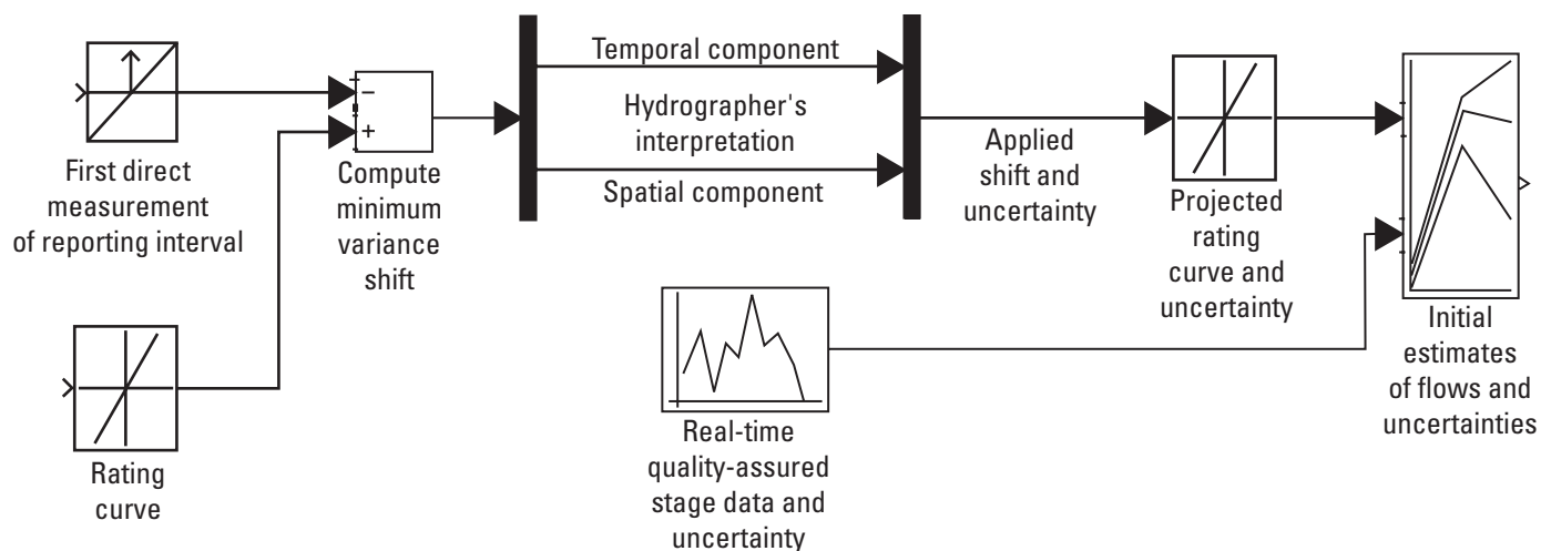
Figure 3. Process for computing initial streamflow estimates.
