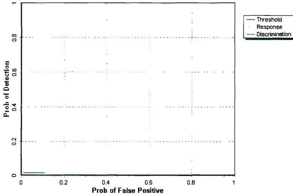
Figure 4. MAG G858/pushcart mogul probability of detection for response and discrimination stages versus their respective probability of false positive for all ordnance larger than 20 mm.
