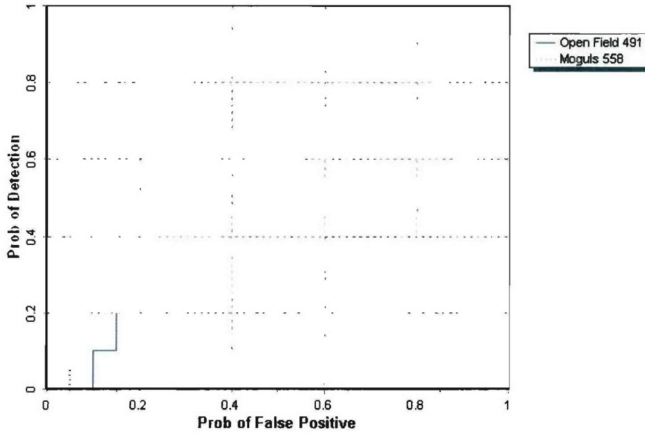
Figure 6. MAG G858/pushcart P_d^{res} stages versus the respective P_{fp} over all ordnance categories combined.
