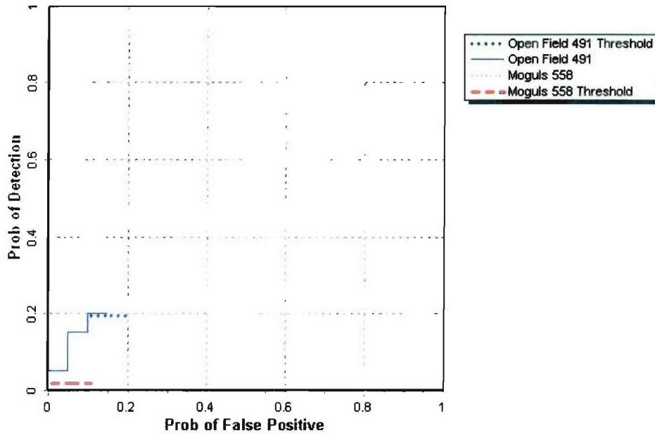
Figure 7. MAG G858/pushcart P_d^{disc} versus the respective P_{fp} over all ordnance categories combined.
