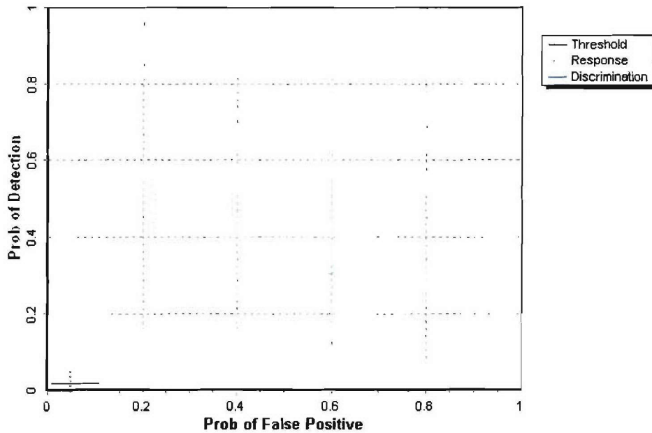
Figure 2. MAG G858/pushcart mogul probability of detection for response and discrimination stages versus their respective probability of false positive over all ordnance categories combined.
