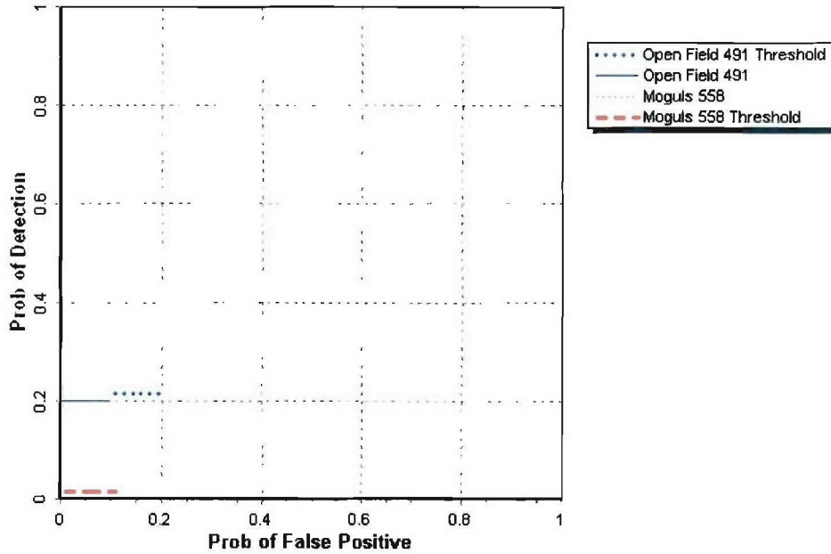
Figure 9. MAG G858/pushcart P_d^{\text{disc}} versus the respective P_{\text{fp}} for ordnance larger than 20 mm.
