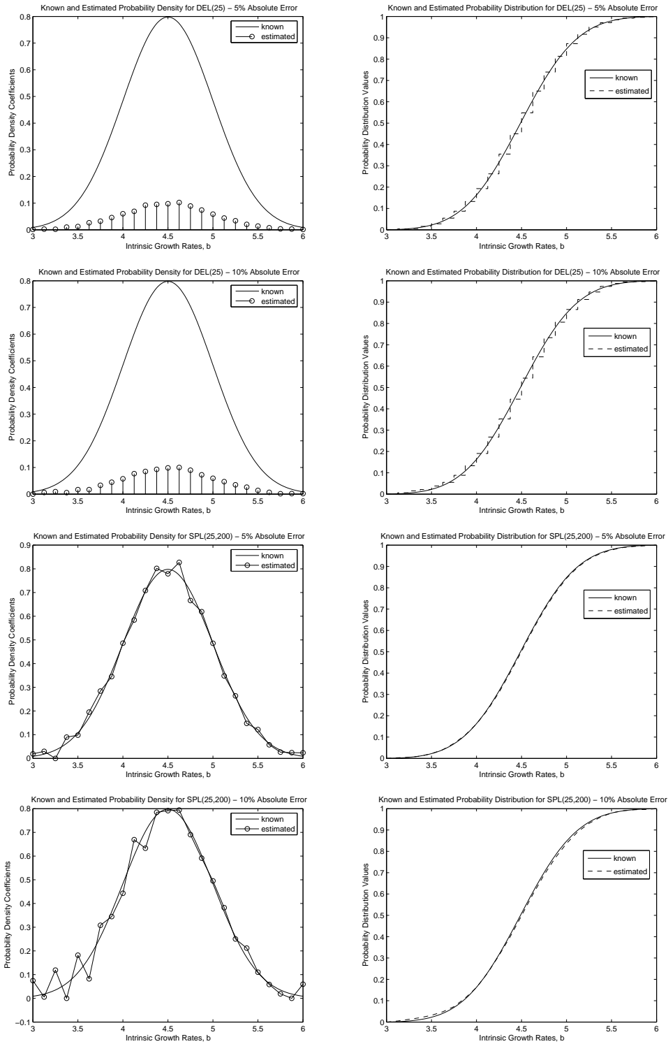
Figure 3: Estimates of probability densities and distributions for true gaussian distribution using a) DEL(25) with 5% absolute error, b) DEL(25) with 10% absolute error, c) SPL(25,200) with 5% absolute error, d) SPL(25,200) with 10% absolute error
