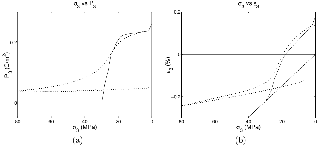
Figure 12: (a) Macroscopic \sigma_3 - P_3 relation and (b) macroscopic \sigma_3 - \epsilon_3 relation. Homogenized 2-D ferroelastic model (—) and experimental PLZT data (···).
