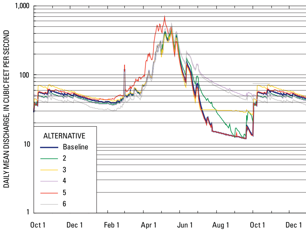
B. Chewuch River at Winthrop (USGS Station 1244800)
