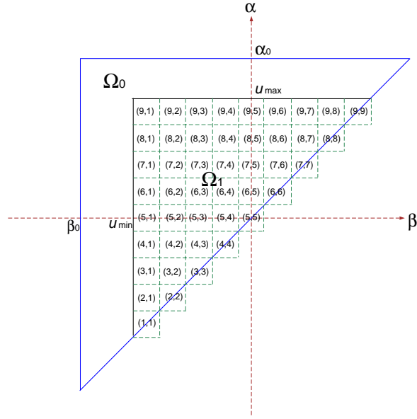
Figure 3. Discretization of the Preisach plane ( L = 9 )
