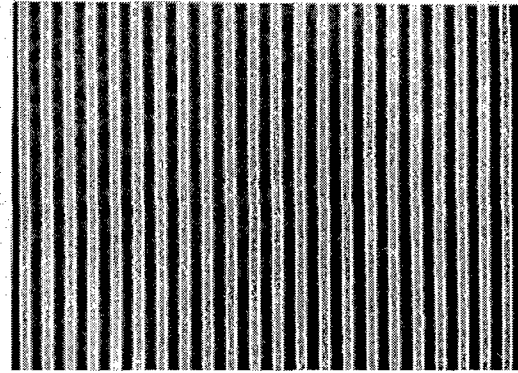
Figure 3. Scanning Electron Micrograph of a surface plasmon enhanced LED showing the metal grating pattern which is used to couple out the radiation.
