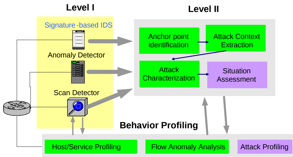
Figure 1: Multi-level Analysis Framework
