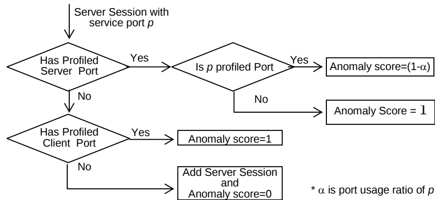
Figure 2. Assigning Anomaly Score to Server session
