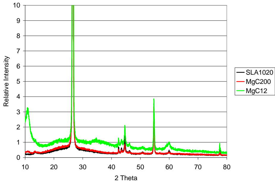
Figure 30: XRD Spectrum of Carbon with Increasing Mg Doping
