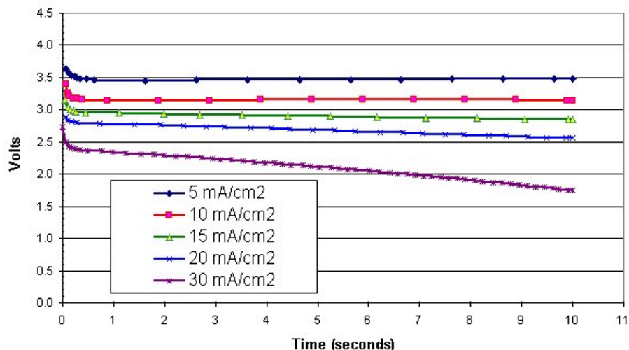
Figure 1: Demonstration of discharge rate capability of \lambda - MnO_2 cathode in a nonaqueous electrolyte solution corresponding to electronic fuse power demand
