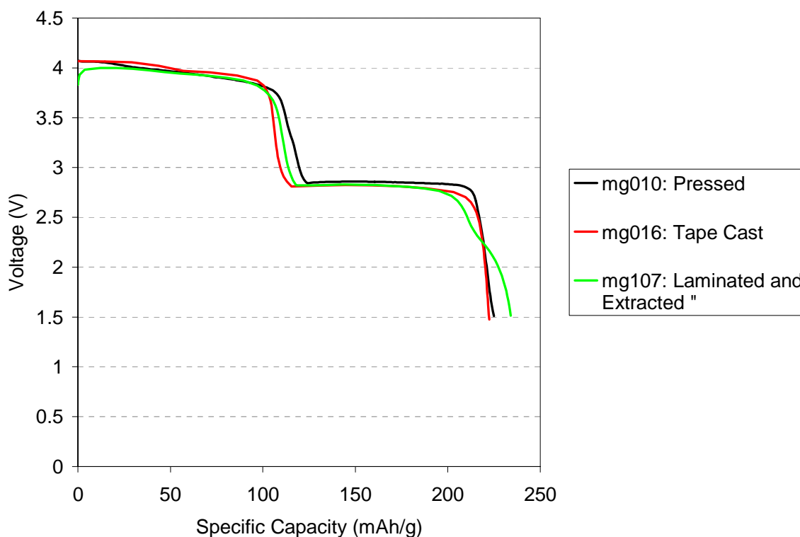
Figure 6: Comparison of \lambda - MnO_2 Thin Film (PVdF) Cells with Thick Film (PTFE) Baseline
