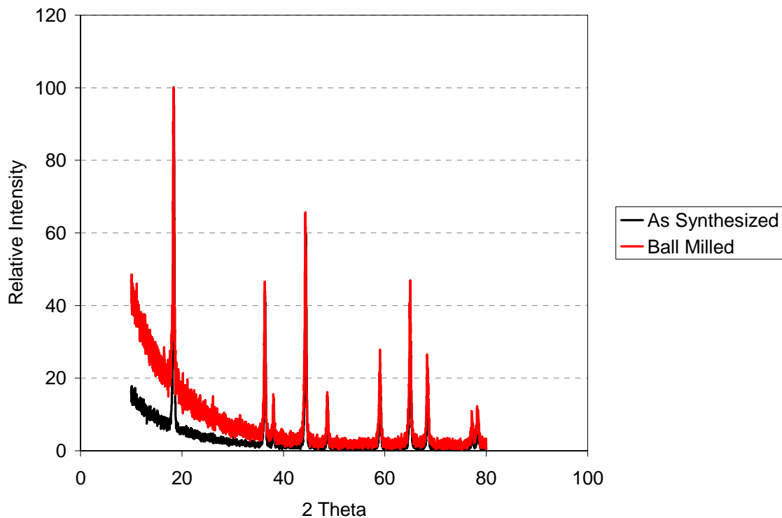
Figure 8: XRD Comparison of Baseline and Ball Milled \lambda - MnO_2
