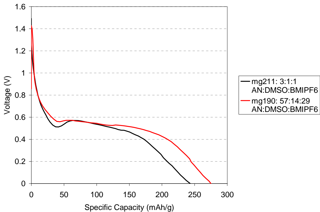
Figure 22: 0.1 \text{ mA/cm}^2 Discharge Voltage Profiles of AZ31B/ \lambda -MnO 2 Cells with Optimized Electrolyte Solutions
