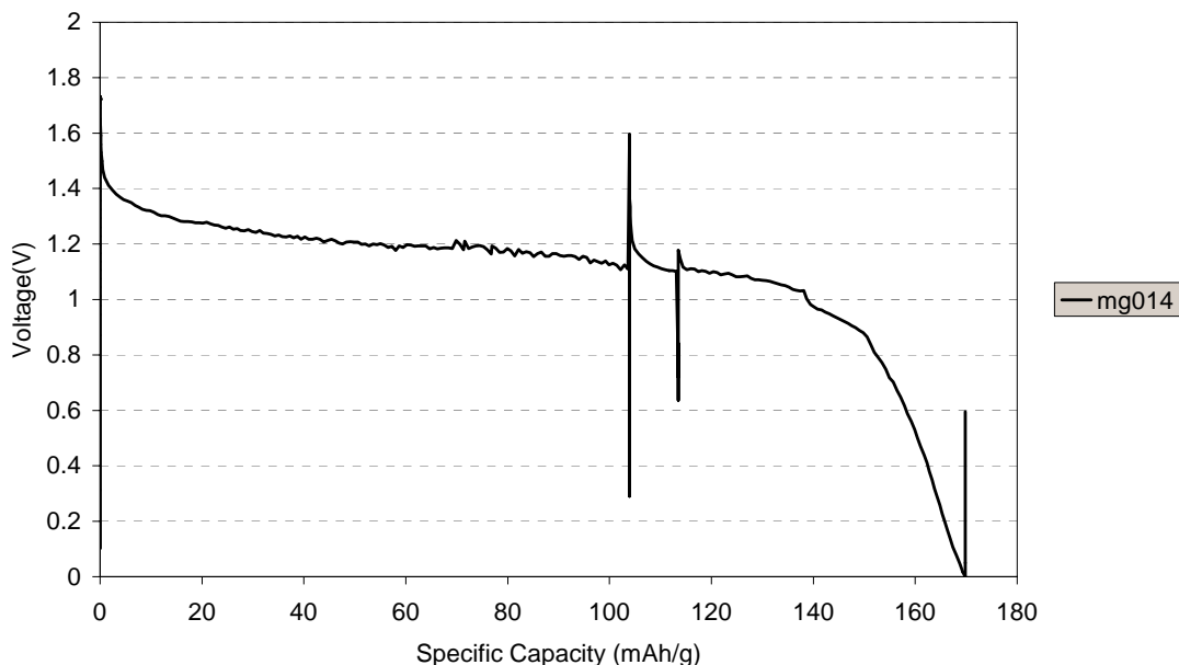
Figure 33: Low Rate Discharge of Mg/ \lambda -MnO 2 Cell
