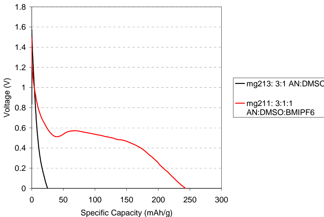
Figure 20: Comparison of Cells with Varying AN:DMSO:BMIPF 6 Ratios at a 0.125 M MgCl 2 Molarity
