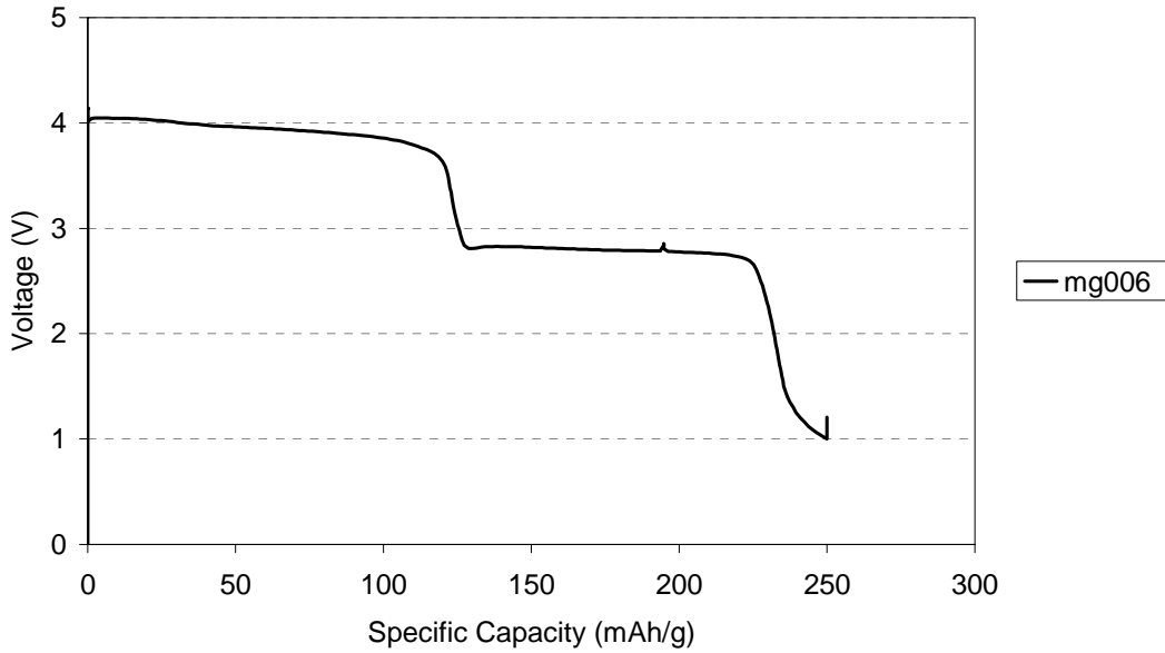
Typical Teflon \lambda -MnO 2 Cathode Discharge Versus Lithium
