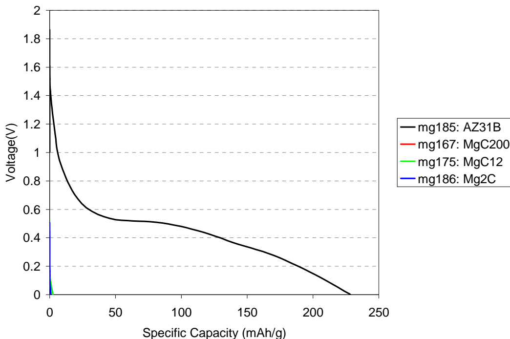
Figure 31 Comparison of Discharge Voltage Profiles of AZ31B Alloy and Mg_xC Powder versus \lambda-MnO_2
