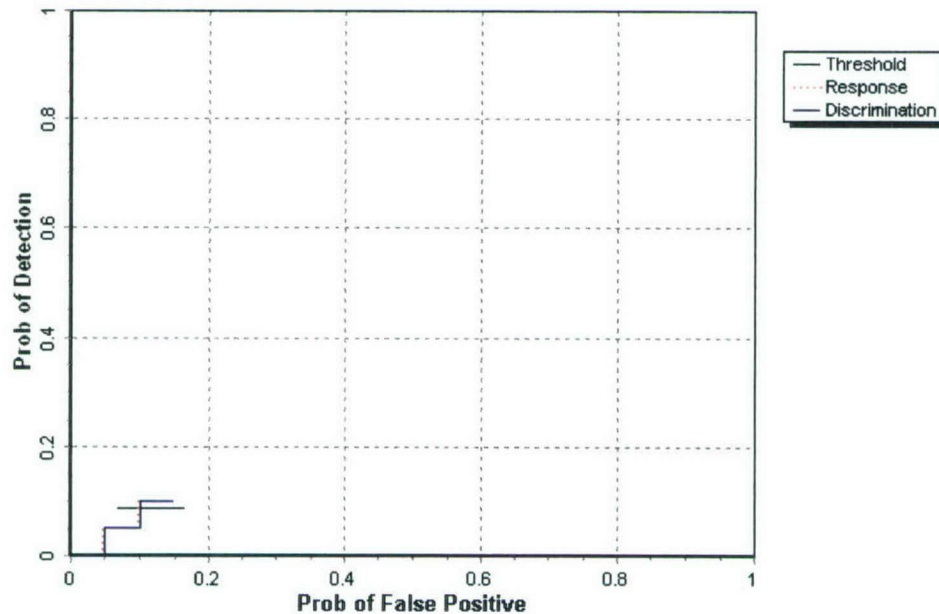
Figure 2. EM61/pushcart desert extreme probability of detection for response and discrimination stages versus their respective probability of false positive over all ordnance categories combined.
