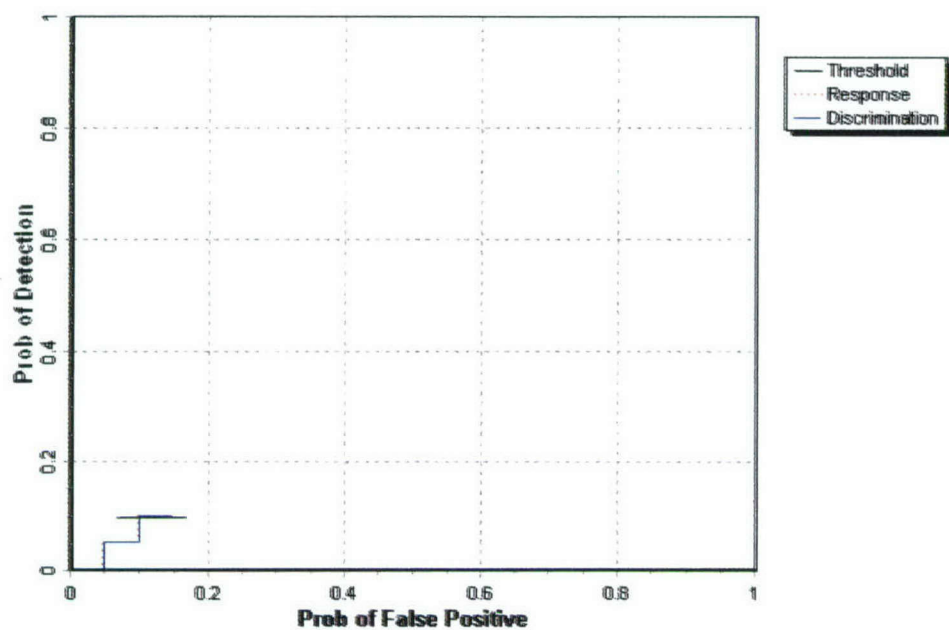
Figure 4. EM61/pushcart desert extreme probability of detection for response and discrimination stages versus their respective probability of false positive for all ordnance larger than 20 mm.
