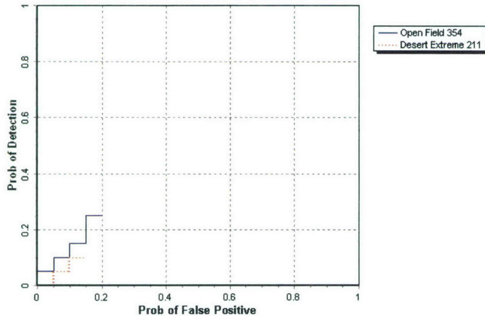
Figure 8. EM61/pushcart P_d^{\text{res}} versus the respective P_{fp} for ordnance larger than 20 mm.
