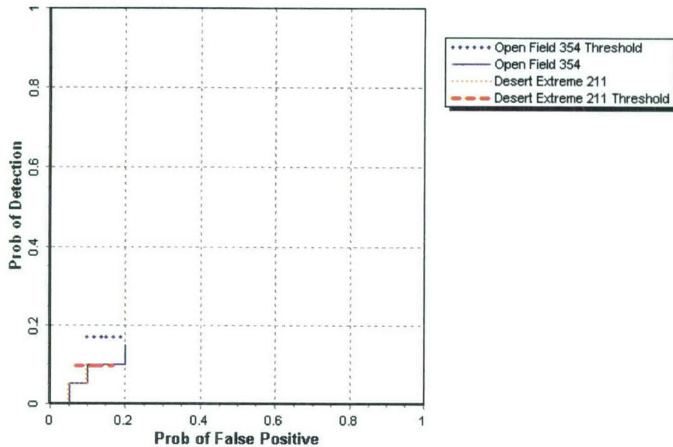
Figure 9. EM61/pushcart P_d^{\text{disc}} versus the respective P_{fp} for ordnance larger than 20 mm.
