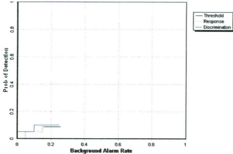
Figure 3. EM61/pushcart desert extreme probability of detection for response and discrimination stages versus their respective background alarm rate over all ordnance categories combined.
