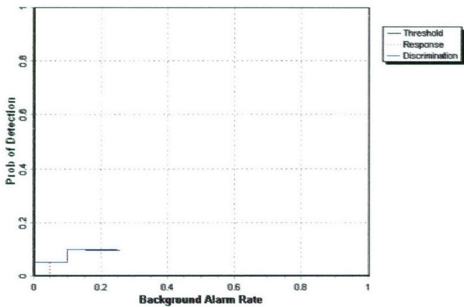
Figure 5. EM61/pushcart desert extreme probability of detection for response and discrimination stages versus their respective background alarm rate for all ordnance larger than 20 mm.
