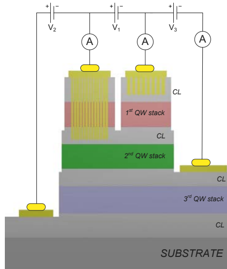
Figure 34 Schematic diagram of the grating configuration to allow three separate photocurrent readouts. The vertical is exaggerated for visual purposes.
