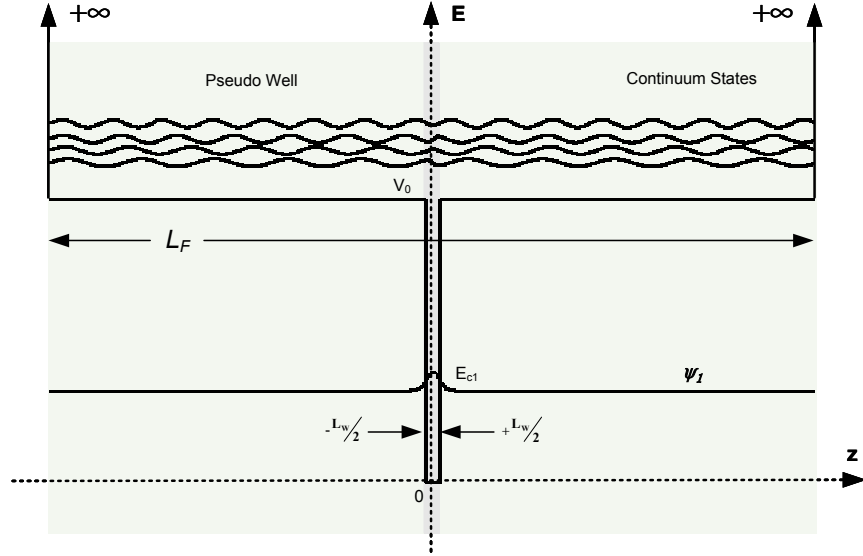
Figure 4 Schematic diagram of the pseudo-quantification technique of the continuous states in of a single square well.
