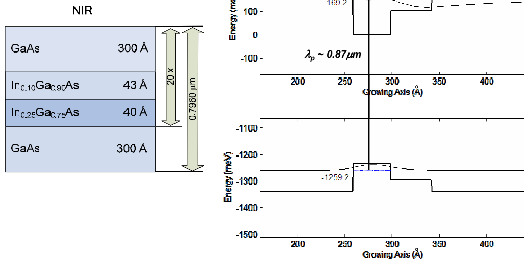
Figure 17 Parameters of the NIR quantum well stack (left) and its respective basic cell potential profile with the confined energy levels (right).
