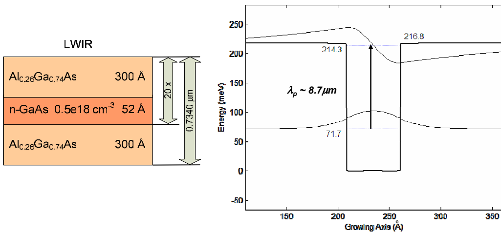
Figure 19 Parameters of the LWIR quantum well stack (left) and its respective basic cell potential profile with the confined energy levels (right).
