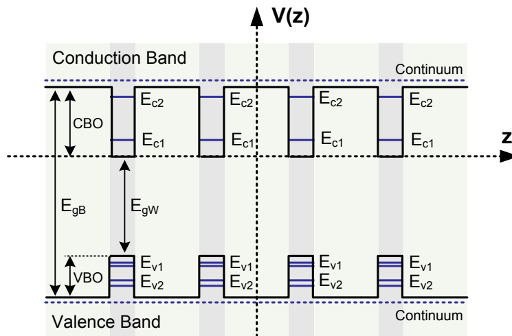
Figure 1 Schematic diagram of a heterostructure potential profile V_e(z) (dark continuous line).
