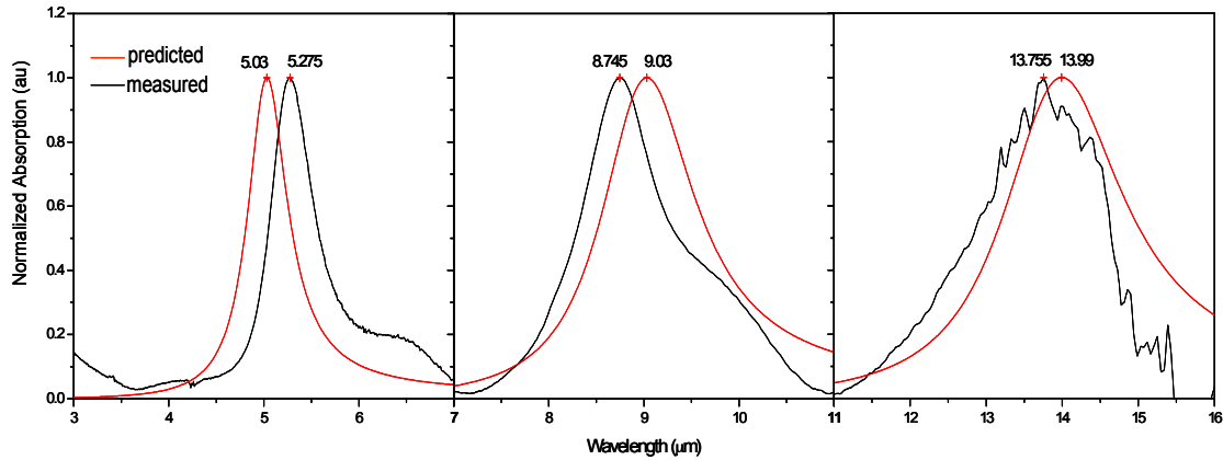
Figure 29 Comparison between the estimated and the measured MWIR and LWIR normalized absorption.
