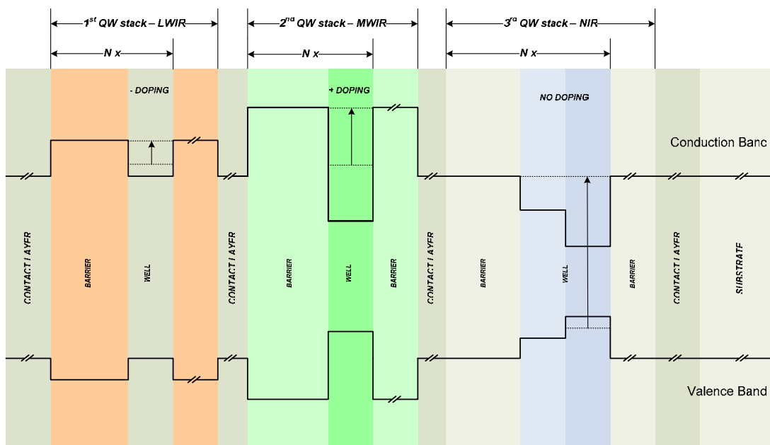
Figure 8 Schematic diagram of the potential profile of the basic detector configuration, including all three quantum well stacks.
