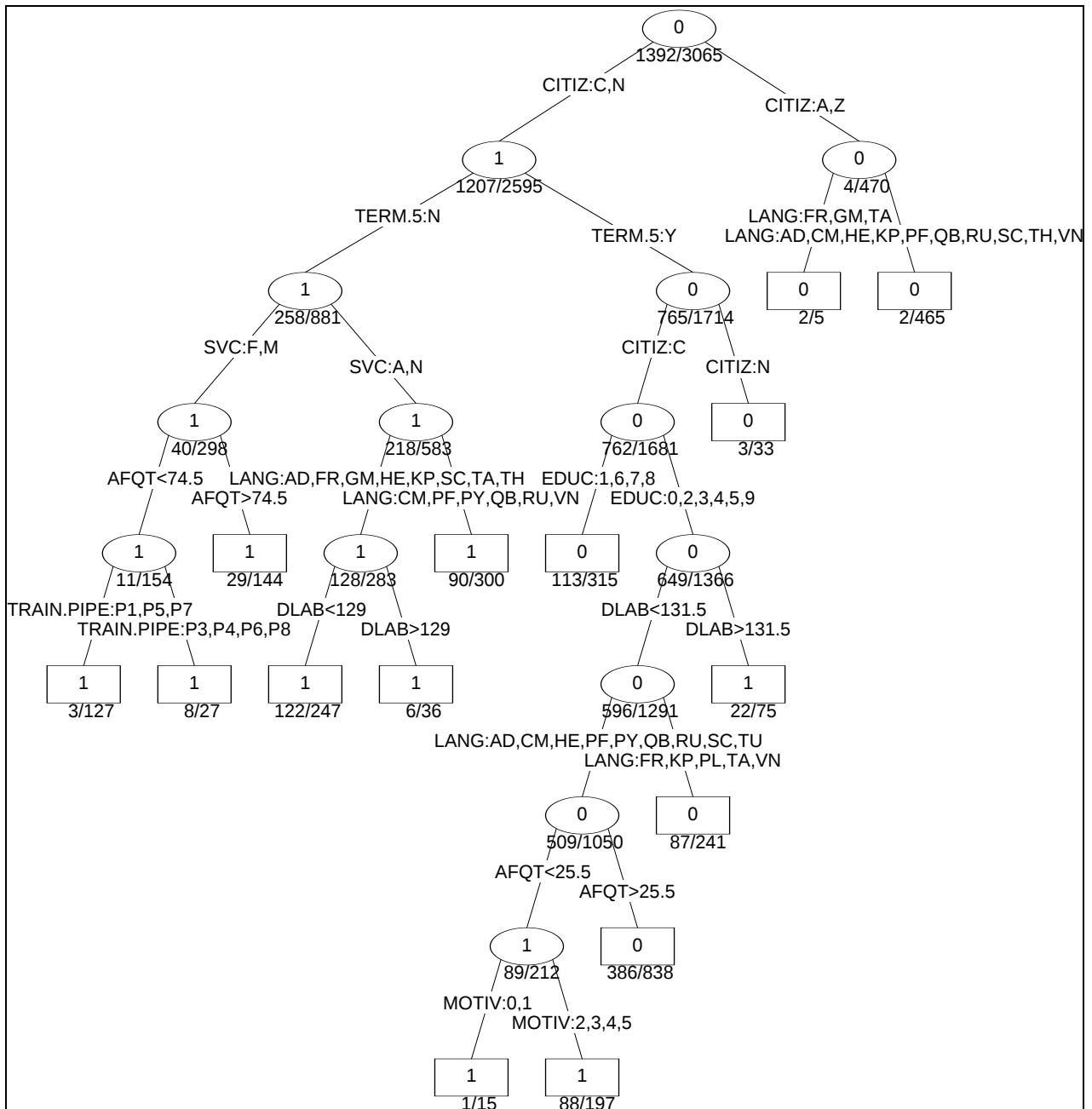
Figure 4.2 Classification Tree
