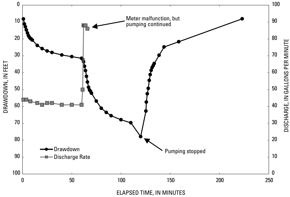
Figure 10. Drawdown and discharge during the November 17, 1998 step-drawdown aquifer test at the Ahoaka Hill monitor well, Kauai, Hawaii.
