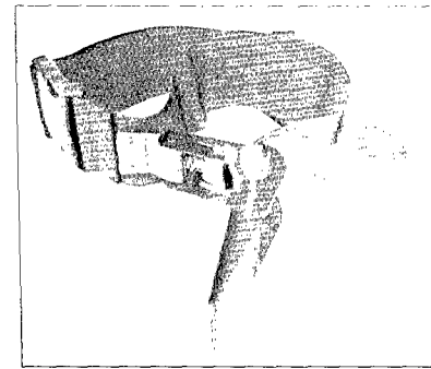
Fig 6. The LRT. The metal portion (similar to a cargo strap) contains a cam-and-ratchet device to tighten the outer strap. This device malfunctioned in some trials.
