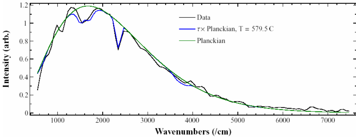
Figure 32. One Planckian Fit to First Kinetic Scan of 0.25 W SiC IR Spectrum Detector resolution of 128\text{ cm}^{-1} was used to collect spectrum. Black curve is raw data. Blue curve represents MATLAB model fitting raw data after atmospheric and detector corrections were applied. Green curve is the Planckian function fit to the data.
