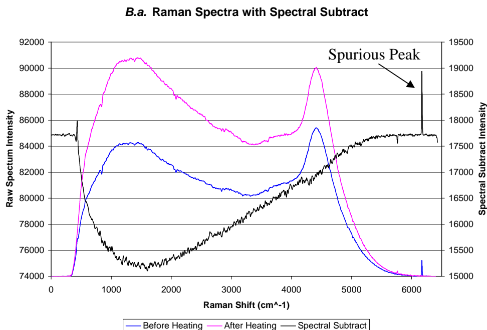
Figure 22. Example of Optical Background Interference with Raman Spectrum
