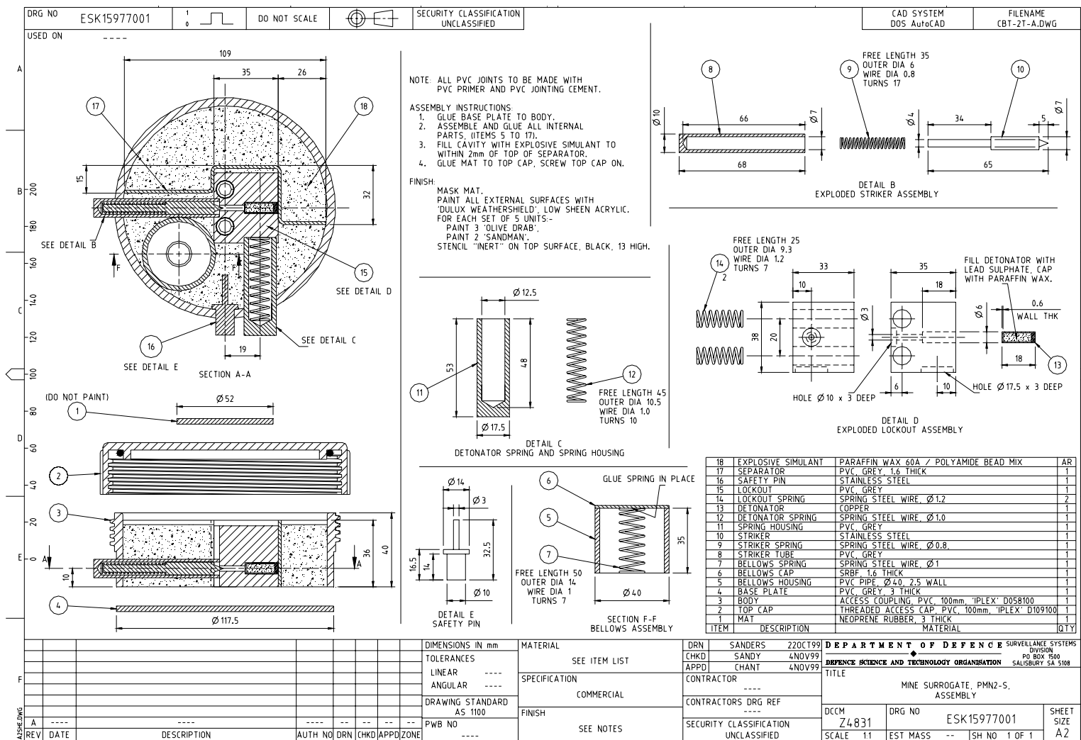
Figure 20: Cutaway drawing of PMN2-S surrogate landmine
