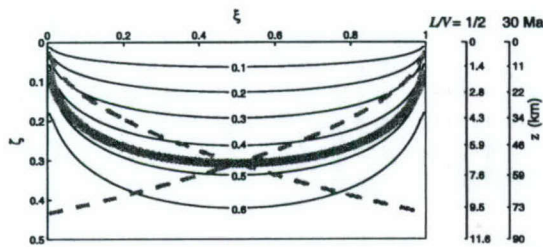
Figure 1. Thermal area of contact, A_T , is the fault area above a reference isotherm T_{ref} . Temperatures of the plates bounding the fault are assumed to evolve as T_0 \text{erf}[\zeta\xi^{-1/2}] and T_0 \text{erf}[\zeta(1-\xi)^{-1/2}] , where T_0 is the mantle potential temperature, \xi = x/L and \zeta = 2/\sqrt{8\kappa L/V} are nondimensionalized length and depth, and \kappa is the thermal diffusivity. Fault isotherms T/T_0 (thin curves) are calculated by averaging the two plate temperatures, which reach a maximum depth in kilometers at z_{max} = 2\sqrt{\kappa L/V} \text{erf}^{-1}(T_{ref}/T_0) . Our model assumes a reference isotherm of T_{ref}/T_0 = 0.46 (thick gray line), or T_{ref} = 600^\circ\text{C} for T_0 = 1300^\circ\text{C} ; the corresponding plate isotherms are plotted as dashed lines. Depth axes for L/V = 0.5 Ma and 30 Ma (right side, in kilometers), calculated for an assumed diffusivity of \kappa = 10^{-12} \text{ km}^2/\text{s} , bound the plate ages spanned by the RTF data set.
