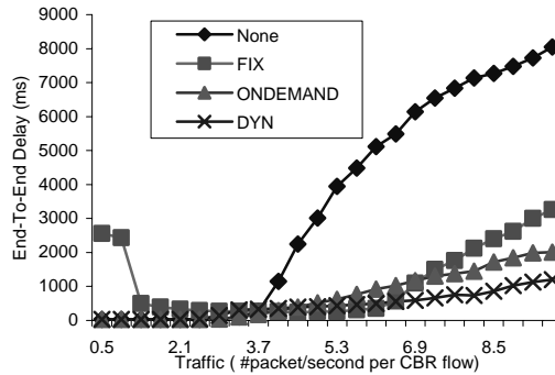
Figure 14: Avg E2E delay (many-to-many 200Kbps)
