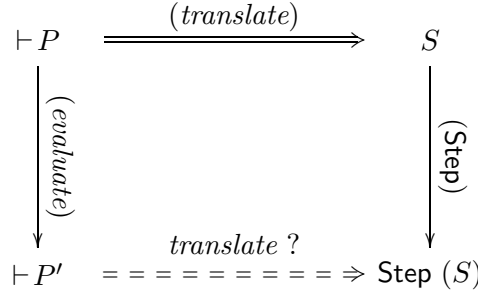
Figure 12. Relationship between FTAL evaluation and machine semantics
