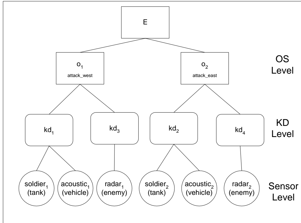
Figure 4 – Graphical Depiction of Example Model M_1
