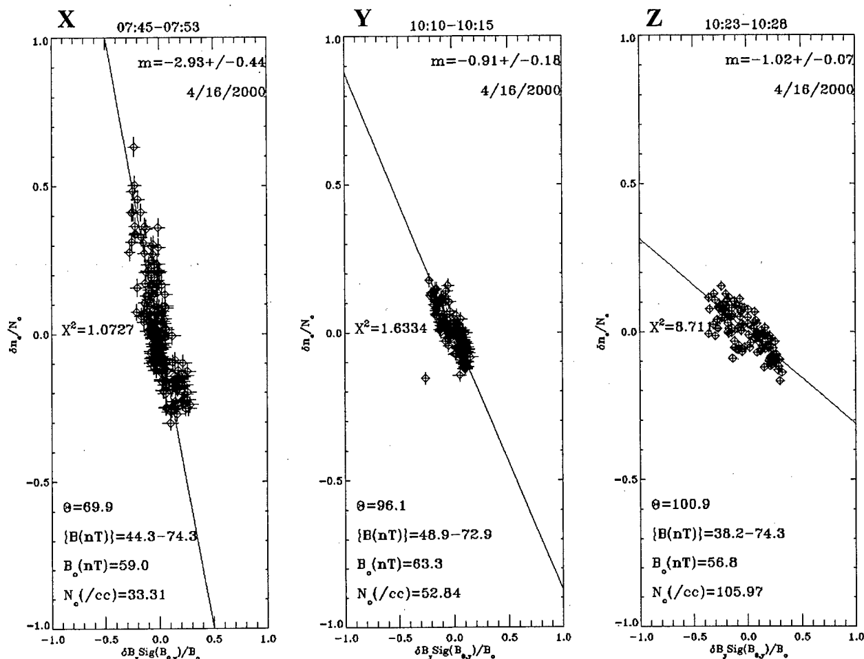
Fig. 12. Linear regression fits for three intervals of 16 April 2000, labeled X, Y, and Z in Fig. 5. See caption for Fig. 11.
