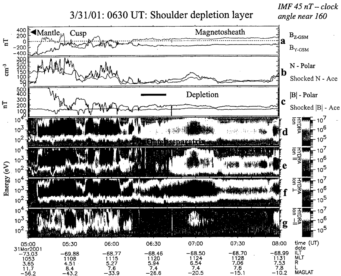
Polar prenoon at -27° MLAT and 1120 MLT – never enters dayside magnetosphere
