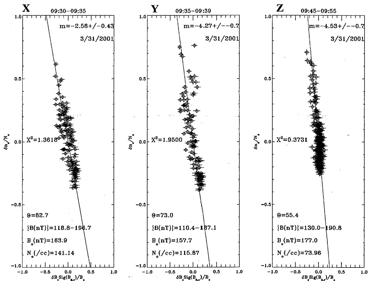
Fig. 11. Linear regression fits for three intervals of 31 March 2001, labeled X, Y, and Z in Fig. 1. Normalized changes in density are plotted as functions of normalized changes in the maximum variance component of B . B_o and N_o represent values of B and N at the nominal fit zero of the plane wave and are constrained to be within the interval. The actual zero may lie outside the interval. The function \text{Sig}(x) , -1 for X < 0 and +1 for X > 0 , is used to rectify the sign of \delta B so that negative values of the resulting slope represent slow-mode solutions. \text{Sig}(0) = 0 . The reported slope m (related to \alpha in Eqs. (1) and (2)) is M/\sin(\Theta_b k) , where M represents actual slopes obtained from the plotted lines. See Scudder et al. (2003) for more details.
