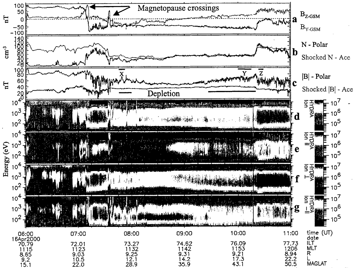
Fig. 5. An example from Polar located prenoon at 30° MLAT and 11:32 MLT in the same format as Fig. 1. The signatures of depletion are seen briefly just before 08:00 UT when IMF B_y is negative and comparable to B_z . Subsequently, as the magnitude of B_y decreases, antiparallel ion fluxes and the total ion density return from merging somewhere below the spacecraft. Depletion is seen on the dusk side of noon for the opposite polarity of B_y near 10:00 UT. Three intervals noted by X, Y, and Z indicate the data on which the regression analyses in Fig. 12 were done.
