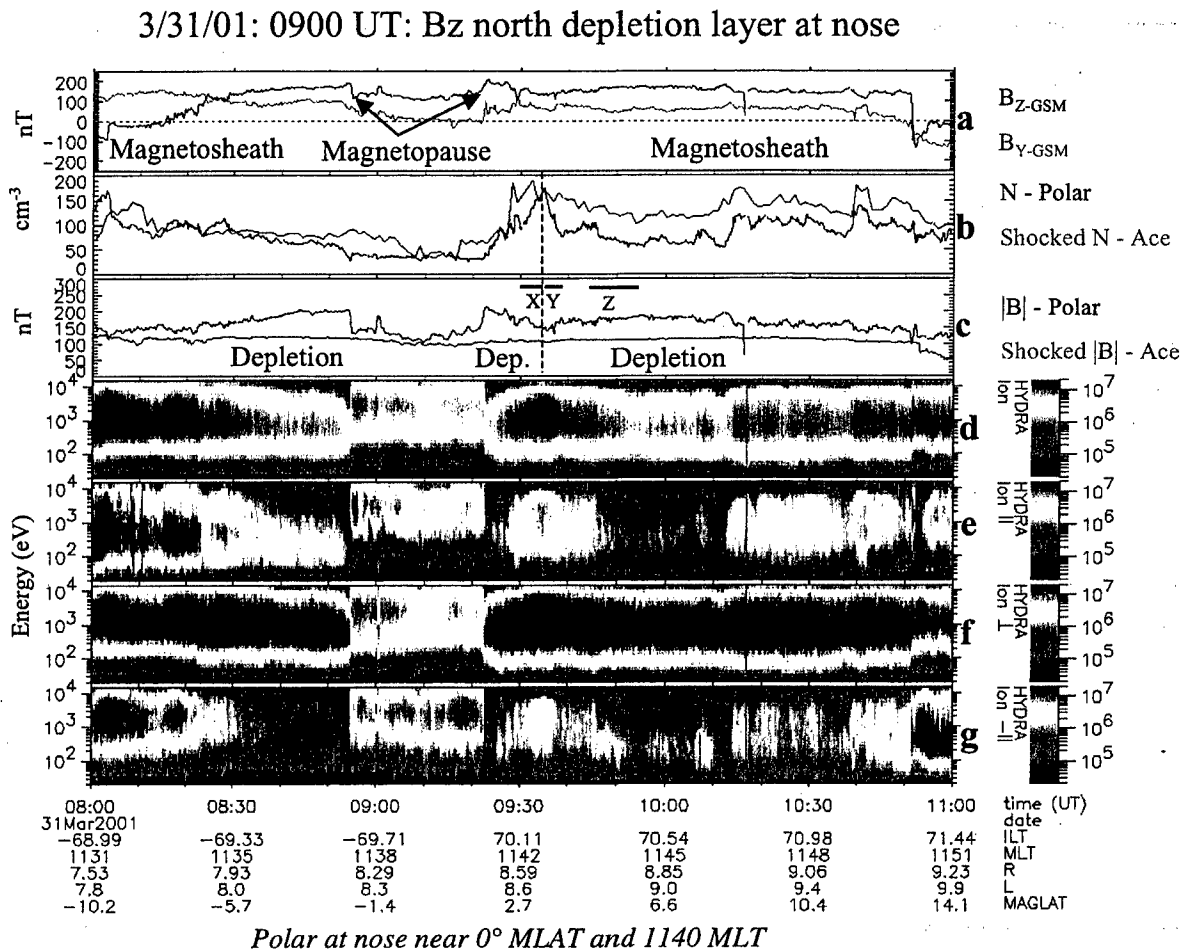
Fig. 1. Example from Polar of depletion layers with IMF B_z northward. Polar was located at 0° MLAT and 11:40 MLT. (a) The black trace is the measured B_z at Polar. The green trace is the measured B_y . The larger value of B_z just outside the magnetopause is a signature of a depletion layer. (b) The measured ion density at Polar (black) compared to the properly lagged (38 min) ion density measured at ACE upstream in the solar wind (blue). Plasma densities attributed to ACE have been multiplied by a time-varying factor appropriate for density jumps predicted by the Rankine-Hugoniot relations for the subsolar bow shock and by an additional compression factor when Polar was close to the magnetopause as predicted by Spreiter and Stahara (1985). (c) The magnetic field magnitude measured at Polar (black) and at ACE (blue). ACE magnetic field measurements were multiplied by the time-varying Rankine-Hugoniot factor appropriate for the magnetic field jumps at the subsolar bow shock. (d–g) Ion energy spectrograms showing the total, parallel (pitch angles 0–30°), perpendicular (75–105°) and antiparallel (150–180°) ion fluxes ( (\text{cm}^2\text{-s-sr-}\Delta E/E)^{-1} ). Three intervals noted by X, Y, and Z indicate the data on which the regression analyses of Fig. 11 were performed.
