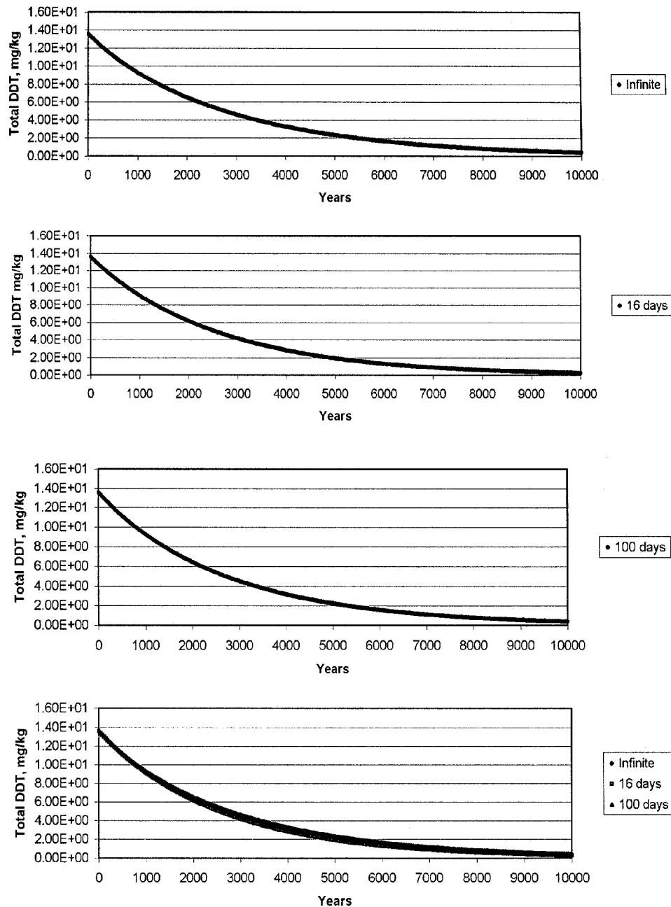
Figure D6. Comparative plots of DDT sediment concentration in the mixed layer, Station 556, showing effect of assumed degradation, no cap condition
