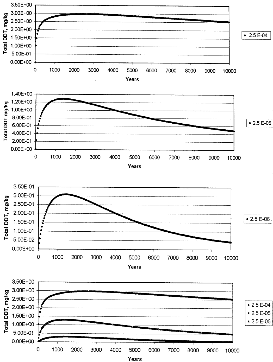
Figure D2. Comparative plots of DDT sediment concentration in the mixed layer, Station 556, showing effect of varying bioturbation coefficient, 15 cm cap
