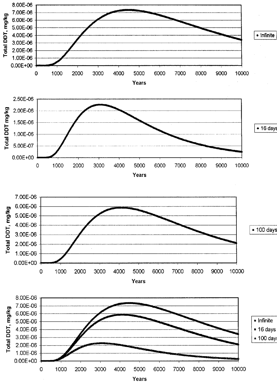
Figure D8. Comparative plots of DDT sediment concentration in the mixed layer, Station 556, showing effects of assumed degradation, 45 cm cap
