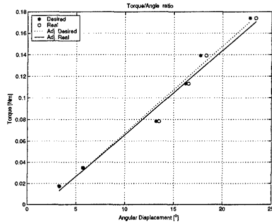
Figure 8: Data exhibiting the linearity of the actuator.
