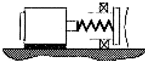
Figure 1: Conceptual depiction of an SEA, comprising a spring in series with a motor.
