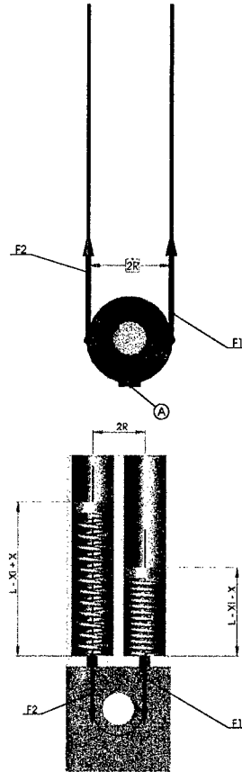
Figure 4: Free body diagrams of the actuator.
