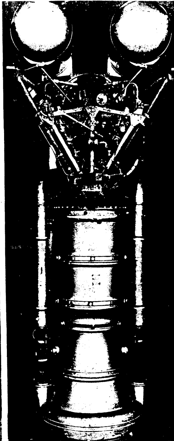
The NAA 75-110 Rocket Engine
