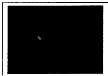
C: L5S2 induced 2h 10nM DHT
