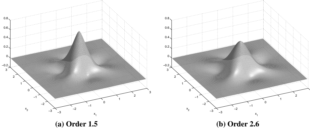
Fig. 1. Example of Polyharmonic B-splines in 2D. Note that they are not compactly supported and decay like O(\|\mathbf{x}\|^{-d-2}) .
