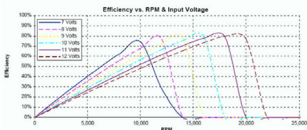
Figure 9 Sample Plot of Modeled Motor Efficiency
