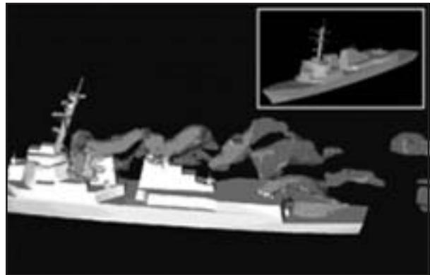
Simulations of temperature isocontours from unsteady airwake simulations over the DDG-51 destroyer were performed in a joint effort with NRL's Tactical Electronic Warfare Division (TEWD).
