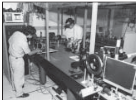
The NRL Table-Top-Terawatt ( T^3 ) Laser Facility. The T^3 laser currently operates at 0.4 ps, 2.5 TW and 5 \times 10^{18} W/cm 2 and provides a facility to conduct research in intense laser-plasma interactions, intense laser-electron beam interactions, and intense laser-matter interactions.
