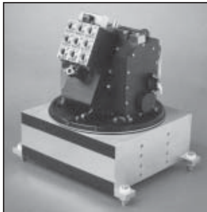
Optical Head Assembly (OHA) of the Polar Ozone and Aerosol Measurement (POAM-II) experiment payload
