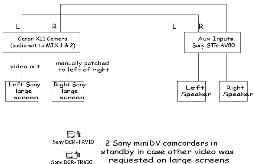
Figure 3.7 – Audio/Video Playback
