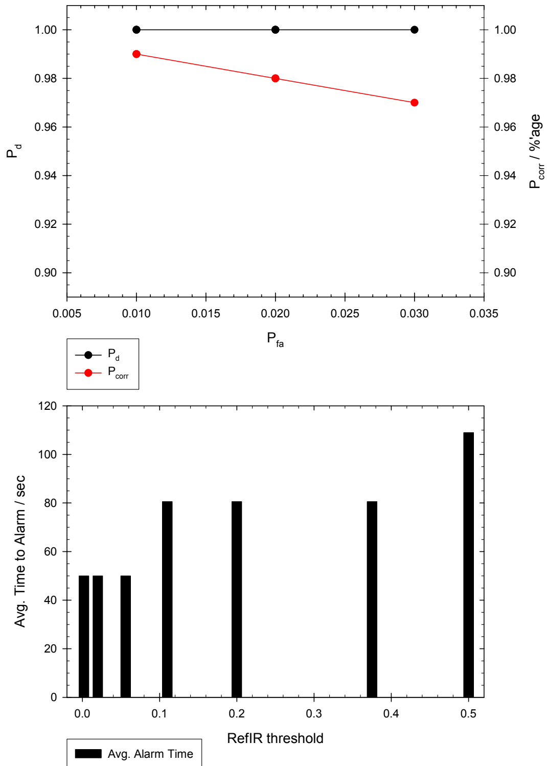
Fig. 6.9 – WELDING RefIR Threshold Optimization Results
