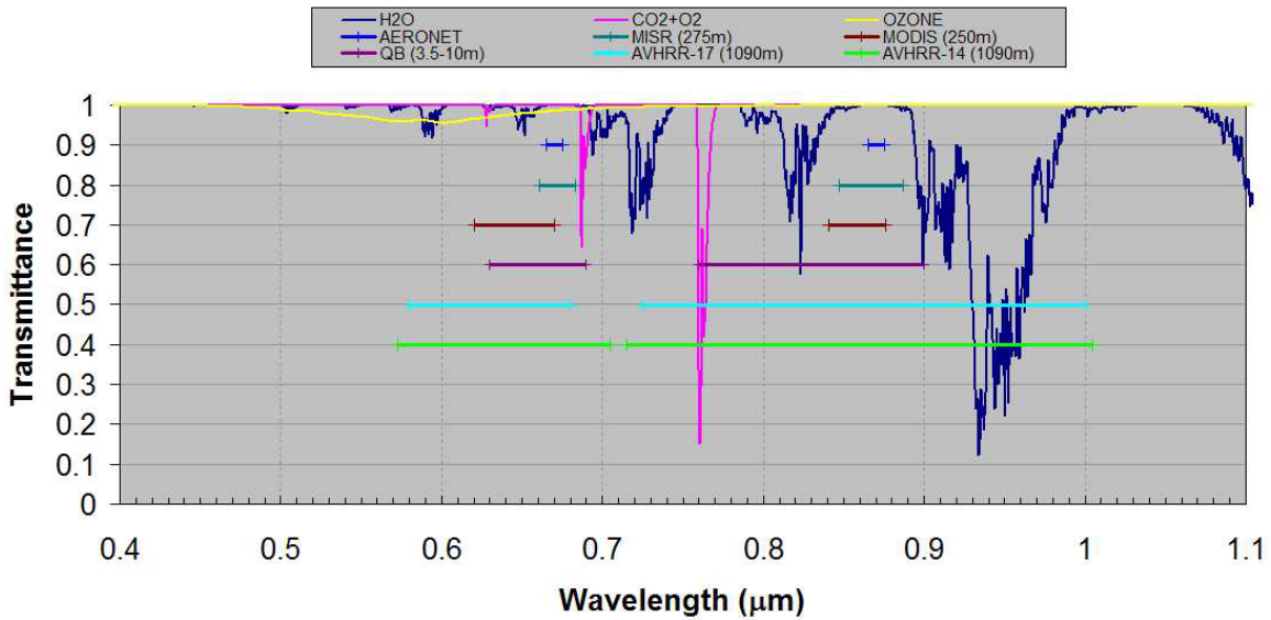
Figure 8. Transmittance as a function of wavelength with applicable sensor bandwidths and atmospheric absorption gases.
