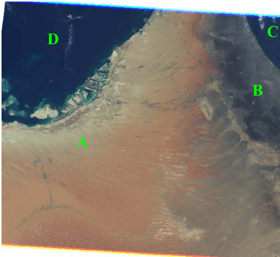
Figure 4. MISR true color image indicating areas of significant red modal radiance peaks
