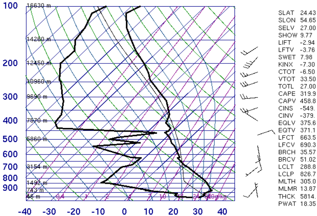
Figure 11. Abu Dhabi, UAE 00Z 19 Sep 2004 sounding indicating an inversion near 925 mb or 700 m (From University of Wyoming 2004).
