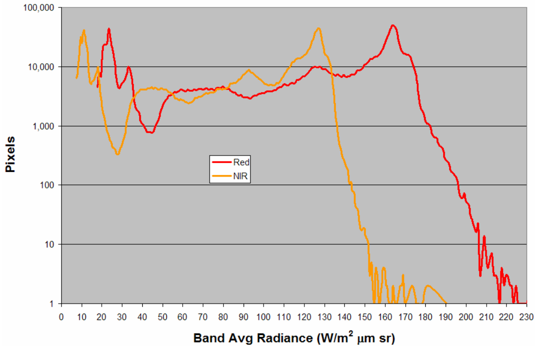
Figure 3. MISR full-scene red and NIR band histograms
