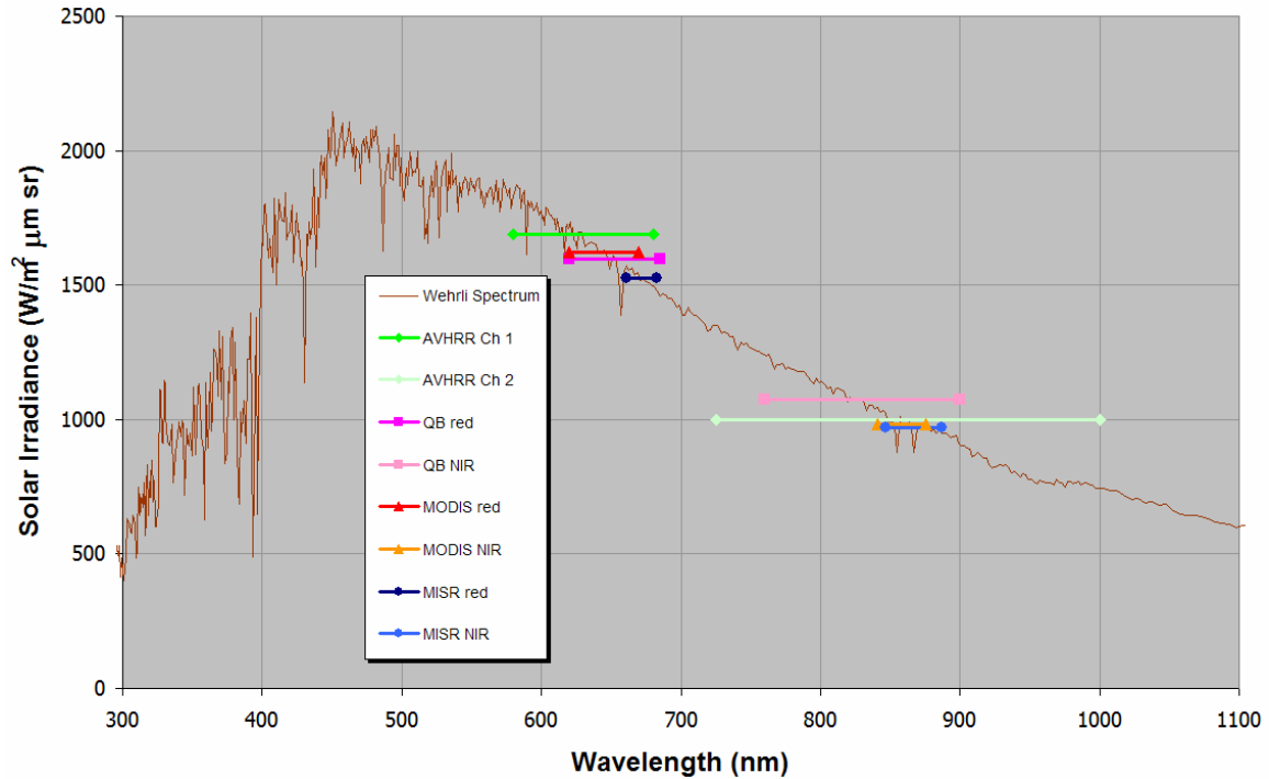
Figure 6. Wehrli solar irradiance spectrum with applicable satellite bandwidths.
