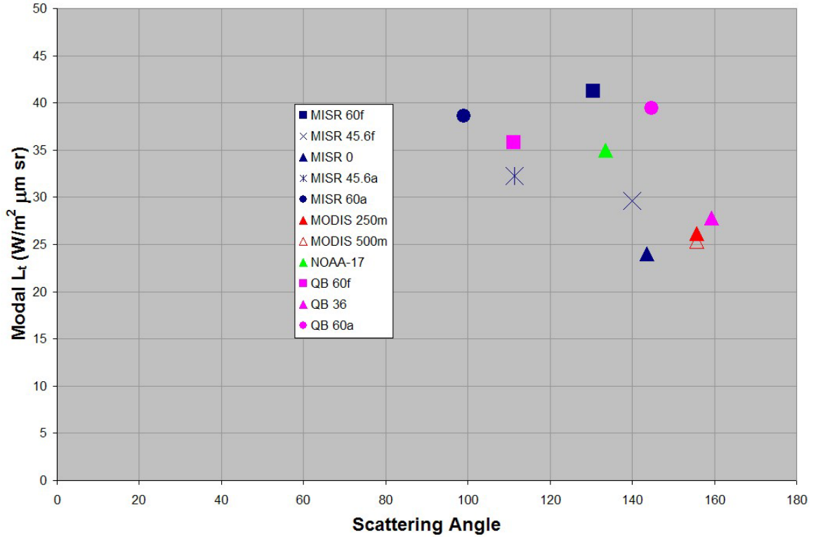
Figure 7. Red modal top of the atmosphere radiance ( L_r ) vs. scattering angle
