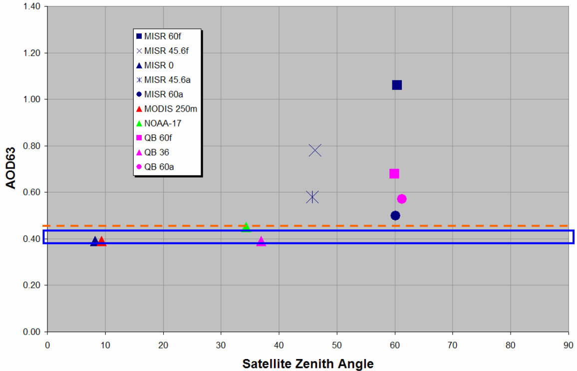
Figure 13. NPS AOD63 (red band) calculated values versus satellite zenith angle. The dashed line indicates the MISR AOD value and the box shows the SBN AERONET estimated AOD range.
