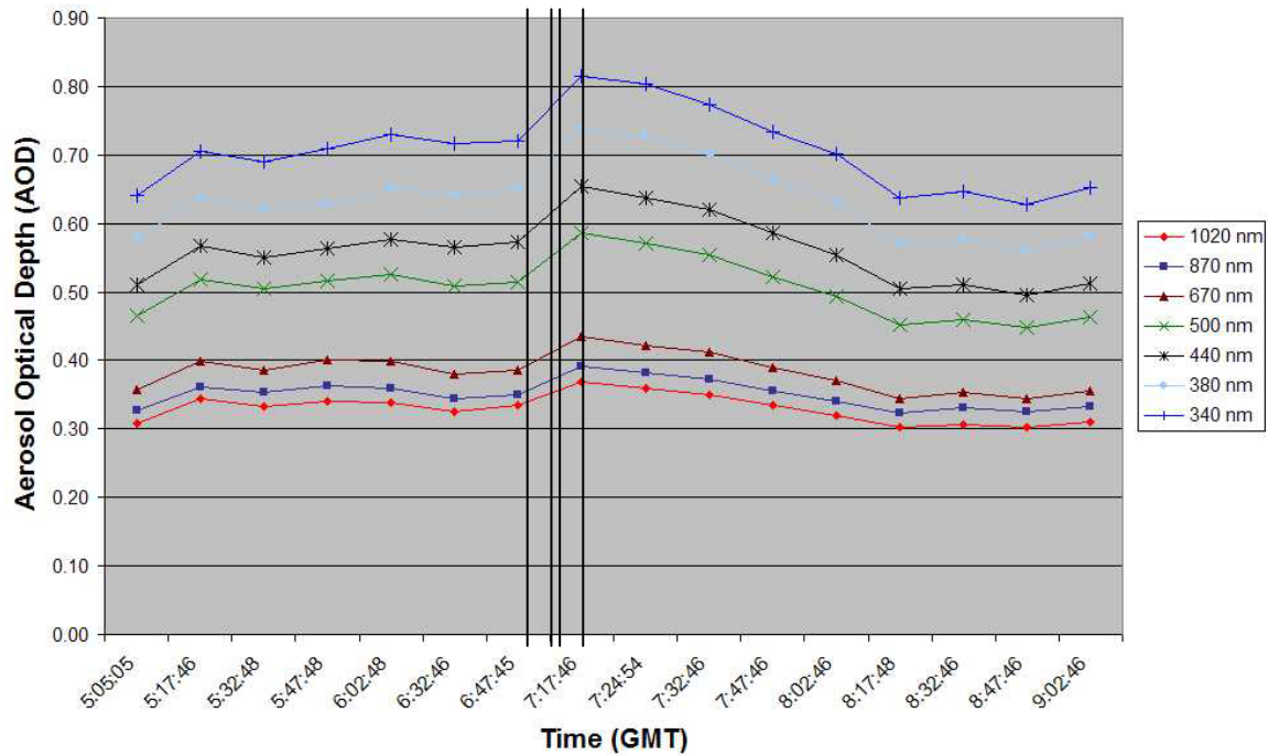
Figure 12. AERONET estimated AOD values at seven wavelengths from 0500-0900Z. Vertical lines, from left to right, indicate satellite overpass times for QB, MODIS, MISR, and AVHRR, respectively.
