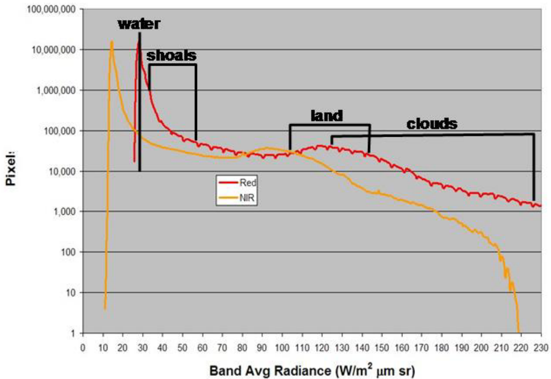
Figure 5. QuickBird nadir view red and NIR band histograms with annotated observed radiances.
