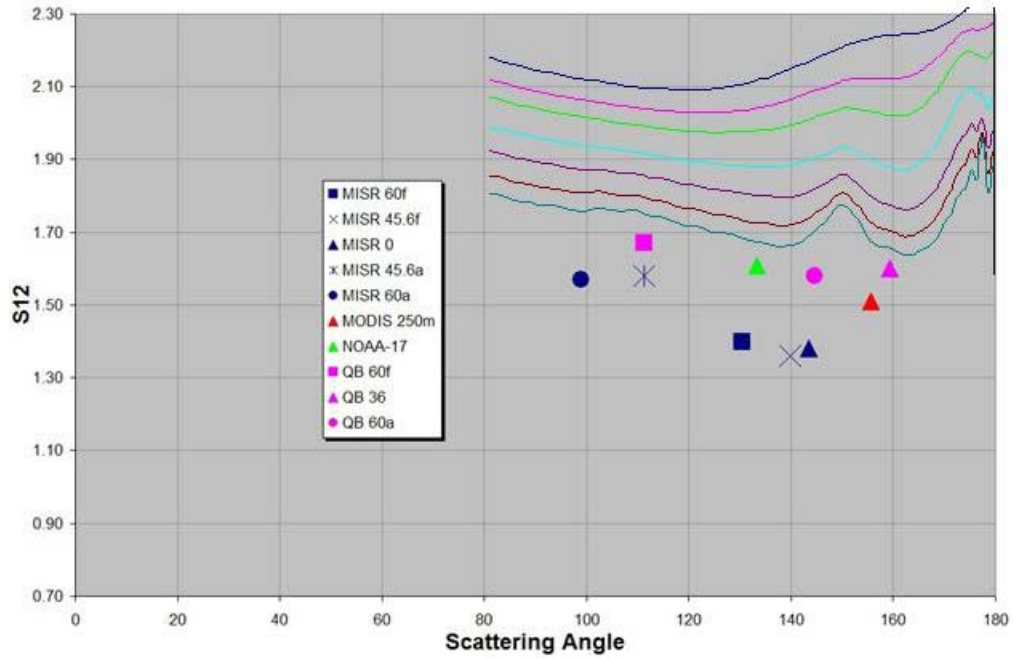
Figure 14. S12 Size Index versus Satellite Scattering Angle with Brown (1997) Aerosol Model Size Distributions
