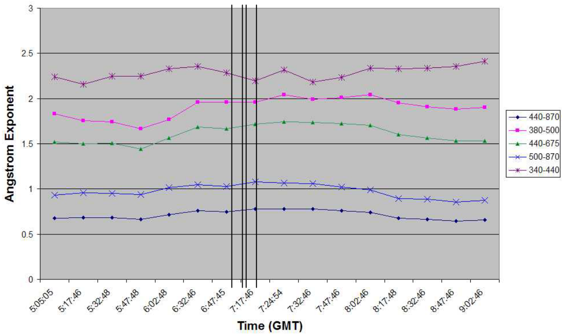
Figure 15. Angstrom Exponent estimated by AERONET between 0500-0900Z
