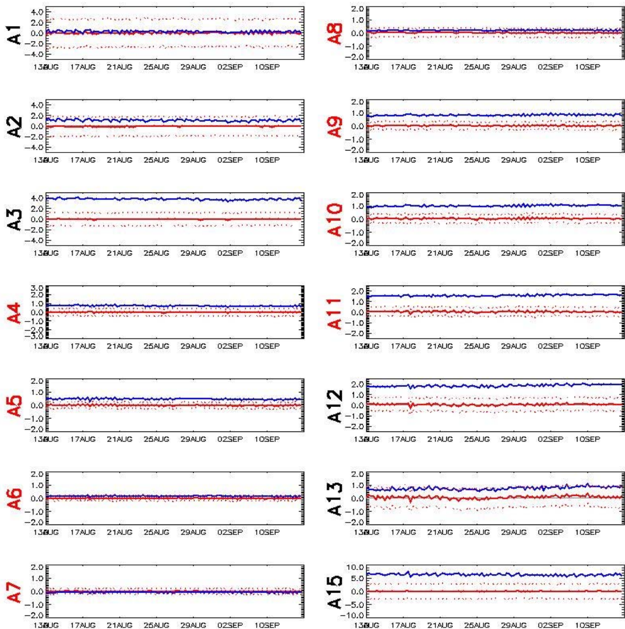
FIG. 20. Example of a radiance bias-monitoring diagram NOAA-16 AMSU-A channels 1 – 15, for a one-month period. The solid blue lines are the uncorrected brightness temperature innovations (observed minus computed), while the solid red lines are the bias corrected innovations. The dotted red lines are the standard deviations of the bias corrected innovations. Red channel numbers indicate that the channel is assimilated by NAVDAS while black channel numbers indicate that the channel is not assimilated (but may be used for QC). Brightness temperature innovations are in Kelvin.
