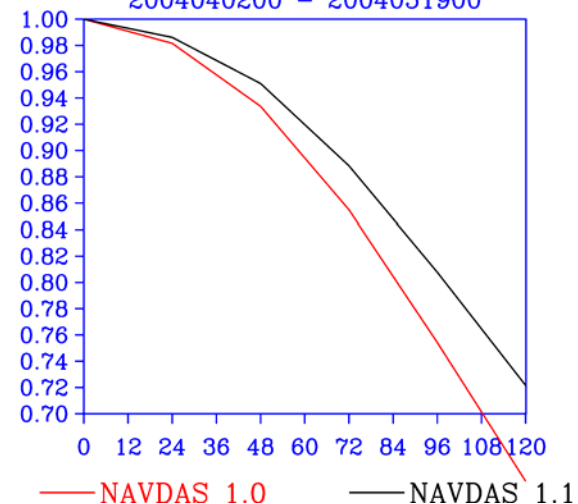
FIG. 16. Same as FIG. 14. for 1000 hPa height.
