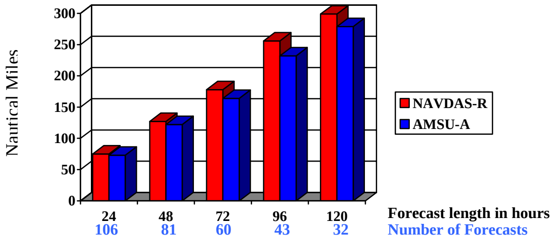
FIG. 18. A comparison of the mean tropical cyclone track error vs. forecast hour for the month of September 2003. The numbers below the forecast time are the total number of forecast tracks for the month used in the comparison. The test run (AMSU-A) includes NAVDAS assimilation of AMSU-A radiances as described in Section 2. The control run (NAVDAS-R) assimilated NESDIS ATOVS retrievals with NAVDAS.
