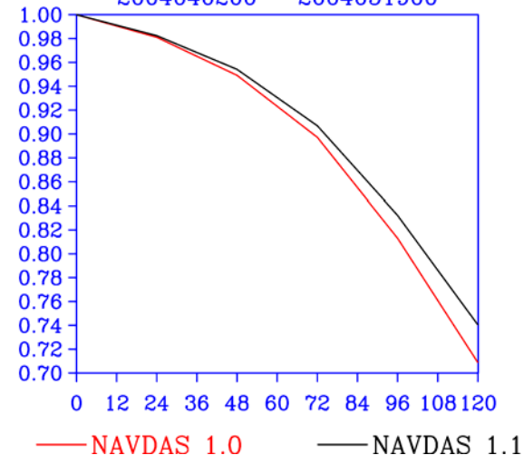
FIG. 17. Same as FIG. 16. for the Northern Hemisphere.
