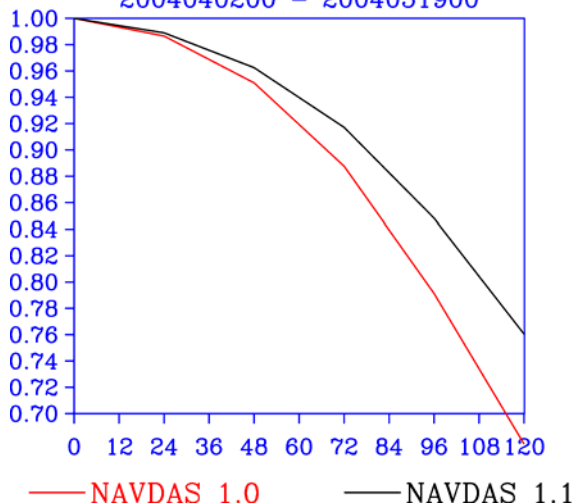
FIG. 14. Southern Hemisphere 500 hPa height AC vs. forecast hour for the April/May 2004 pre-operational test period. NAVDAS 1.1 includes AMSU-A radiances, while NAVDAS 1.0 used NESDIS ATOVS retrievals.
