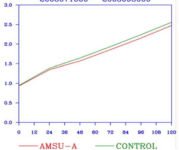
FIG. 8. The 700 hPa temperature rms error with respect to radiosonde vs. forecast hour for the summer 2003 case. The test run (AMSU-A) includes NAVDAS assimilation of AMSU-A radiances as described in Section 2. The control run assimilated NESDIS ATOVS retrievals with NAVDAS.
