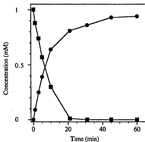
FIG. 4. Conversion of 3HAP (■) to aminohydroquinone (●) by 3HAP mutase from R. eutropha JMP134. The enzyme (0.6 U) and 3HAP (1 mM) were incubated in 100 mM phosphate buffer (pH 7) under an argon atmosphere at 30°C. The conversion was analyzed by HPLC.
